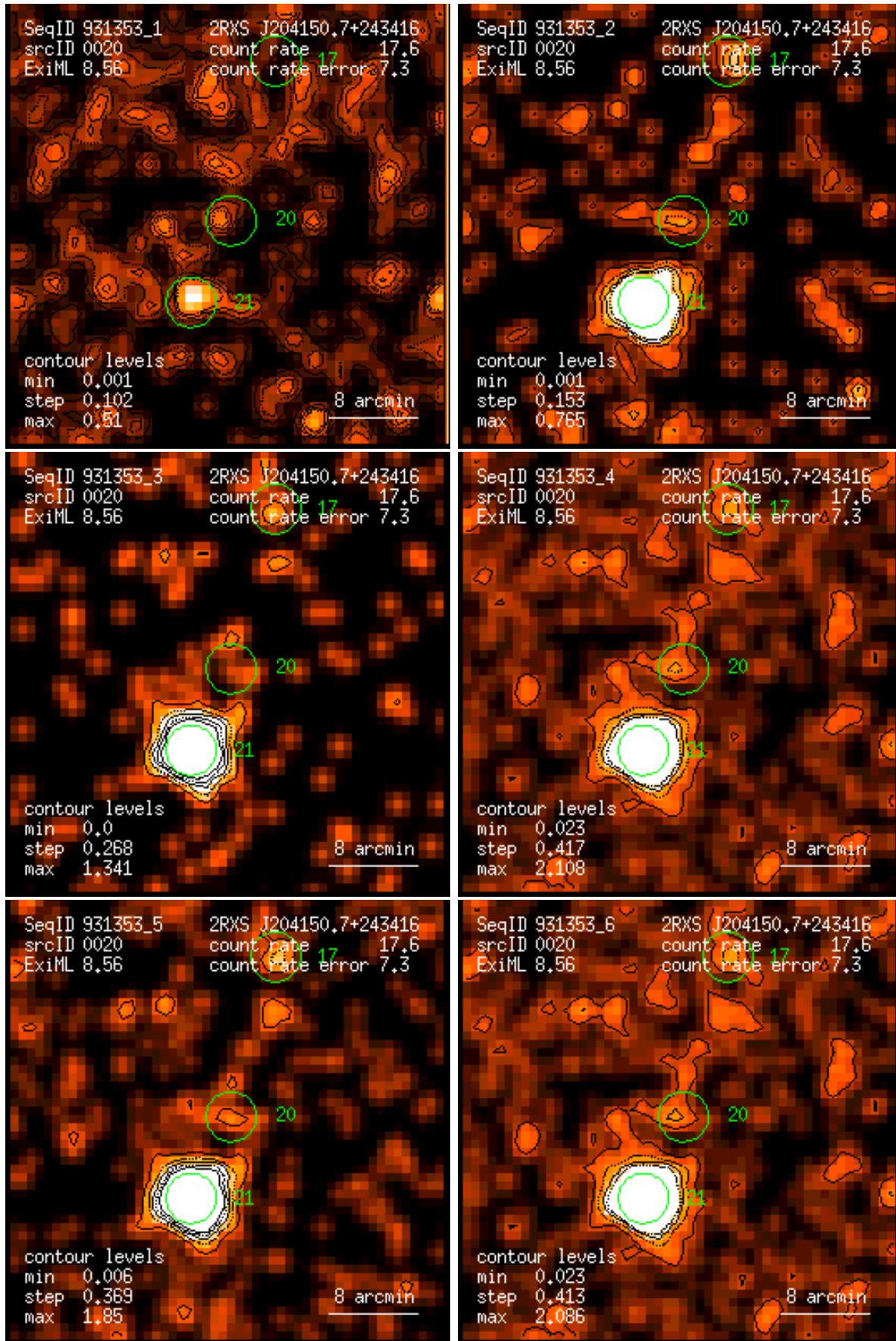
Figure 20: RASS 931353: detection 0020: band rate images, Gaussian filter: (1) PSPC channels 11 – 41, (2) 52 – 90, (3) 91 – 201, (4) 11 – 235, (5) 52 – 201, (6) 11 – 201. Broad band rates in counts/ks. Band rate contour levels in counts/ks/arcmin 2 .
