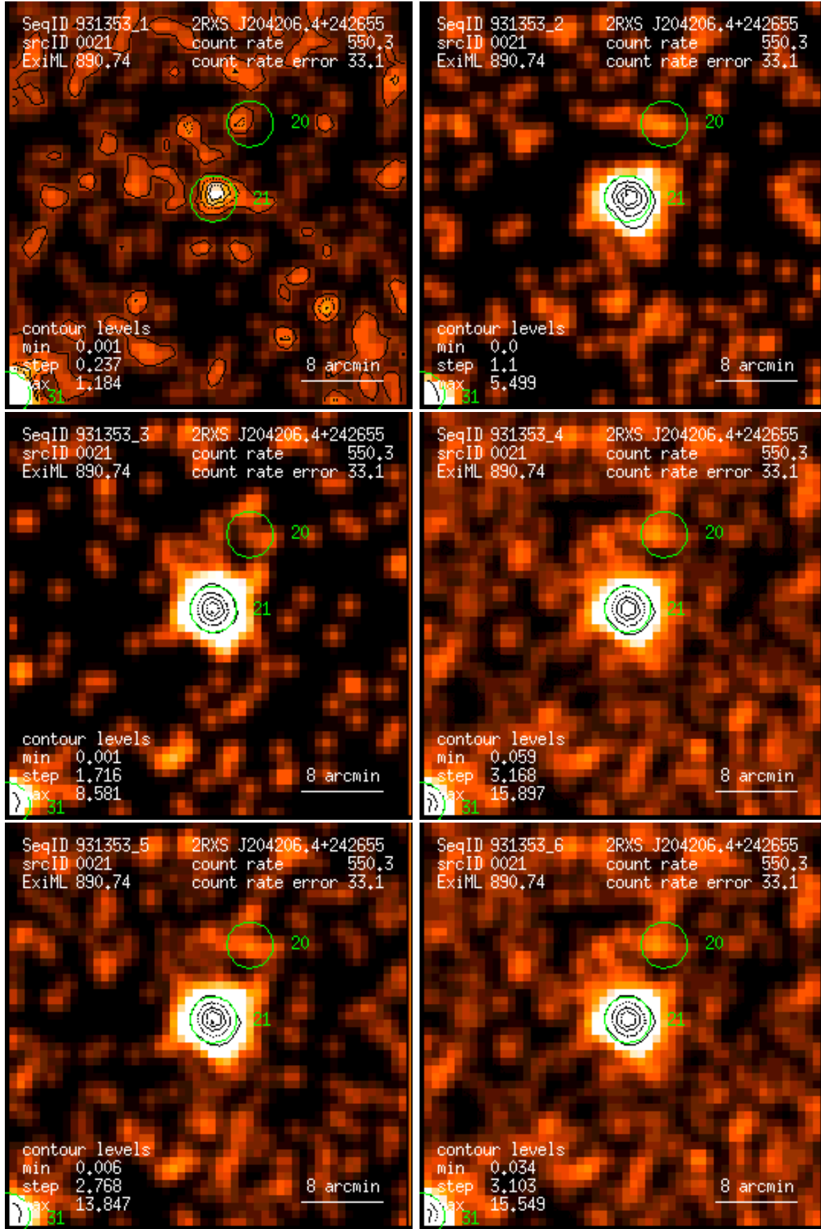
Figure 21: RASS 931353: detection 0021: band rate images, Gaussian filter: (1) PSPC channels 11 – 41, (2) 52 – 90, (3) 91 – 201, (4) 11 – 235, (5) 52 – 201, (6) 11 – 201. Broad band rates in counts/ks. Band rate contour levels in counts/ks/arcmin 2 .
