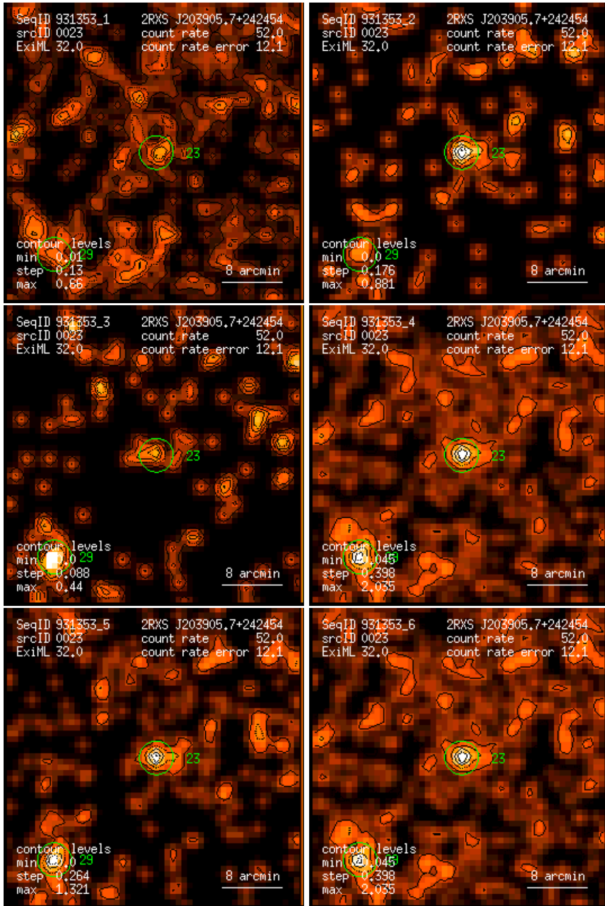
Figure 23: RASS 931353: detection 0023: band rate images, Gaussian filter: (1) PSPC channels 11 – 41, (2) 52 – 90, (3) 91 – 201, (4) 11 – 235, (5) 52 – 201, (6) 11 – 201. Broad band rates in counts/ks. Band rate contour levels in counts/ks/arcmin 2 .
