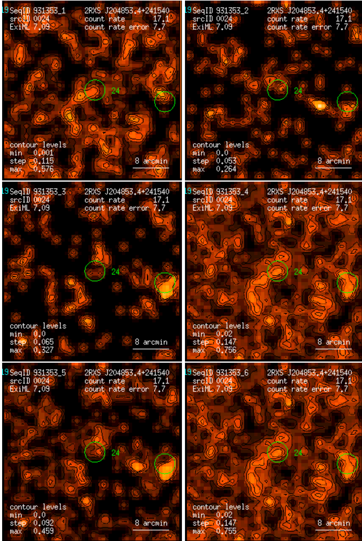
Figure 24: RASS 931353: detection 0024: band rate images, Gaussian filter: (1) PSPC channels 11 – 41, (2) 52 – 90, (3) 91 – 201, (4) 11 – 235, (5) 52 – 201, (6) 11 – 201. Broad band rates in counts/ks. Band rate contour levels in counts/ks/arcmin 2 .
