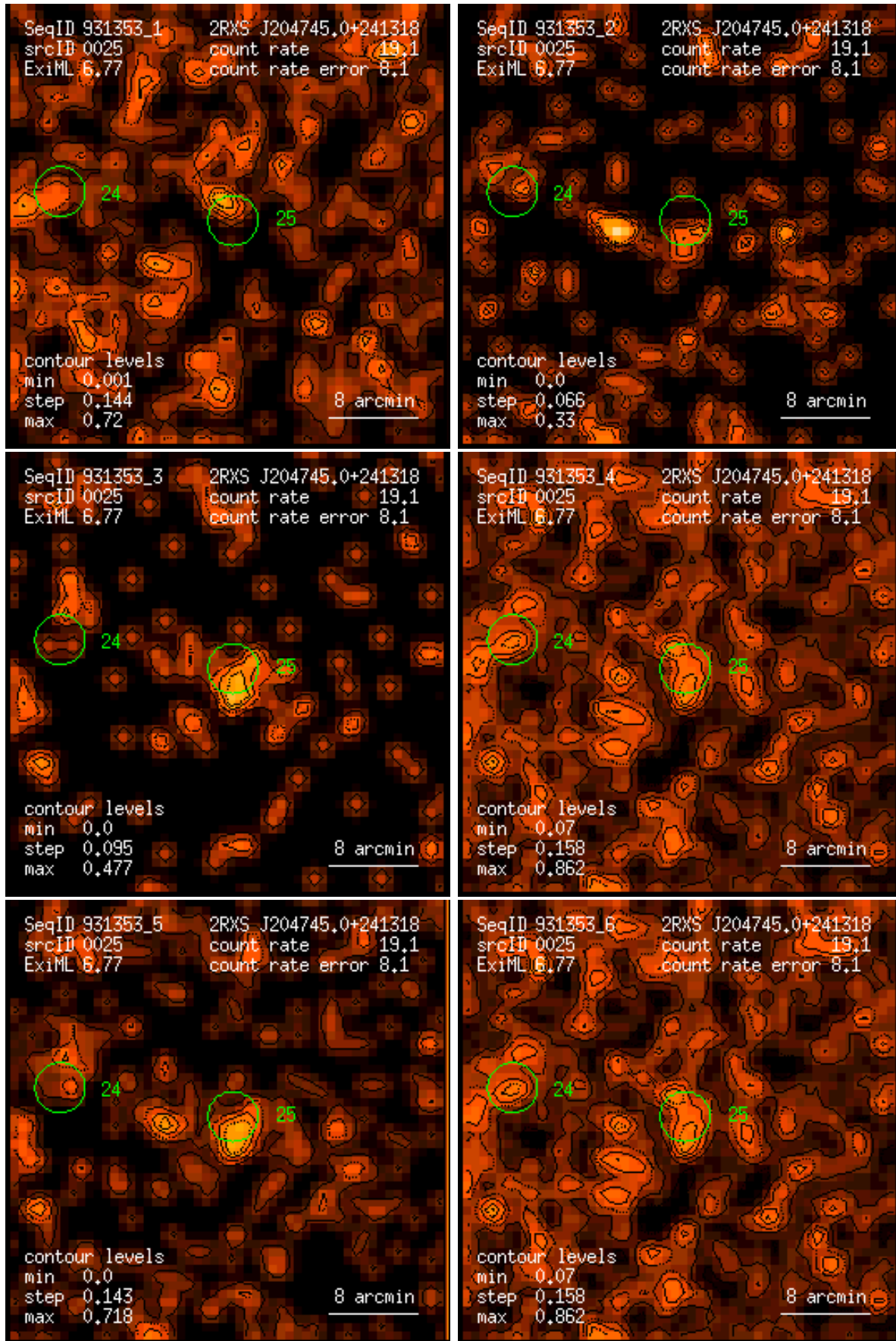
Figure 25: RASS 931353: detection 0025: band rate images, Gaussian filter: (1) PSPC channels 11 – 41, (2) 52 – 90, (3) 91 – 201, (4) 11 – 235, (5) 52 – 201, (6) 11 – 201. Broad band rates in counts/ks. Band rate contour levels in counts/ks/arcmin 2 .
