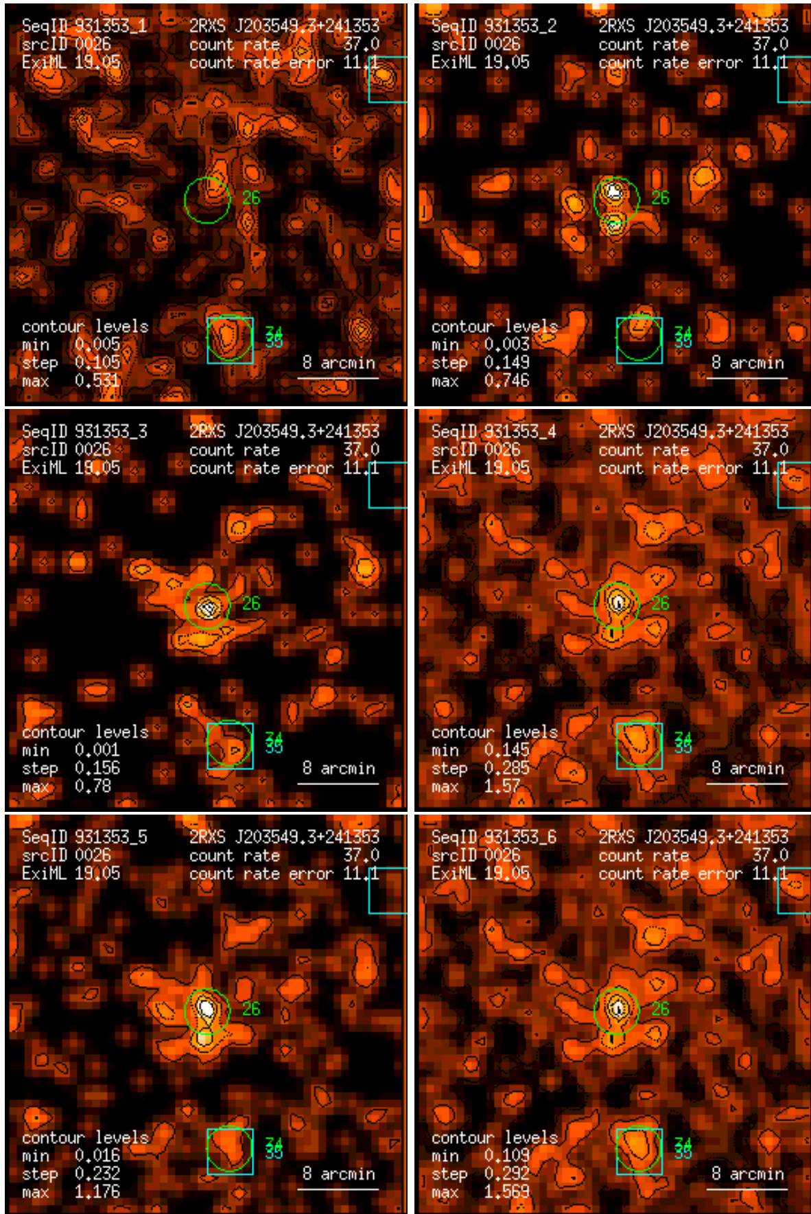
Figure 26: RASS 931353: detection 0026: band rate images, Gaussian filter: (1) PSPC channels 11 – 41, (2) 52 – 90, (3) 91 – 201, (4) 11 – 235, (5) 52 – 201, (6) 11 – 201. Broad band rates in counts/ks. Band rate contour levels in counts/ks/arcmin 2 .
