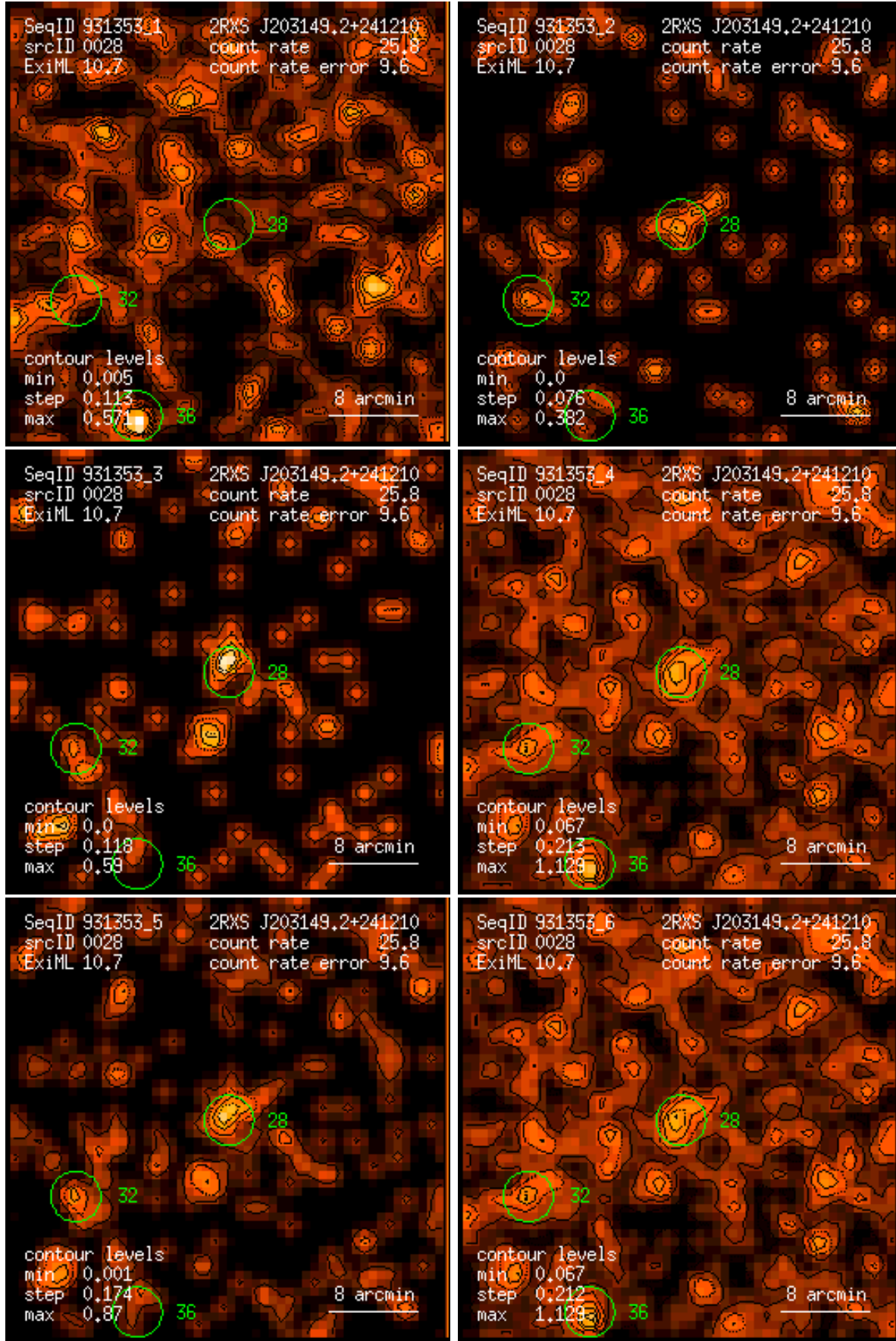
Figure 28: RASS 931353: detection 0028: band rate images, Gaussian filter: (1) PSPC channels 11 – 41, (2) 52 – 90, (3) 91 – 201, (4) 11 – 235, (5) 52 – 201, (6) 11 – 201. Broad band rates in counts/ks. Band rate contour levels in counts/ks/arcmin 2 .
