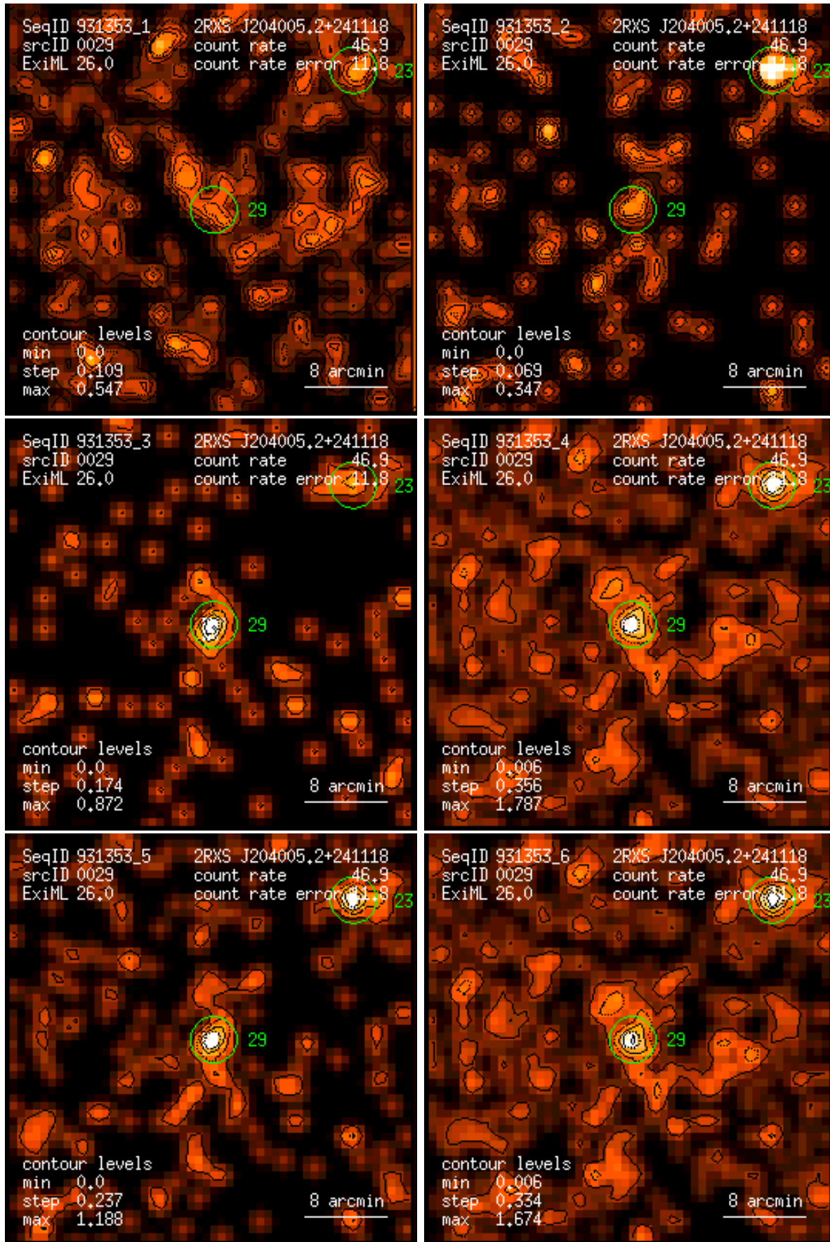
Figure 29: RASS 931353: detection 0029: band rate images, Gaussian filter: (1) PSPC channels 11 – 41, (2) 52 – 90, (3) 91 – 201, (4) 11 – 235, (5) 52 – 201, (6) 11 – 201. Broad band rates in counts/ks. Band rate contour levels in counts/ks/arcmin 2 .
