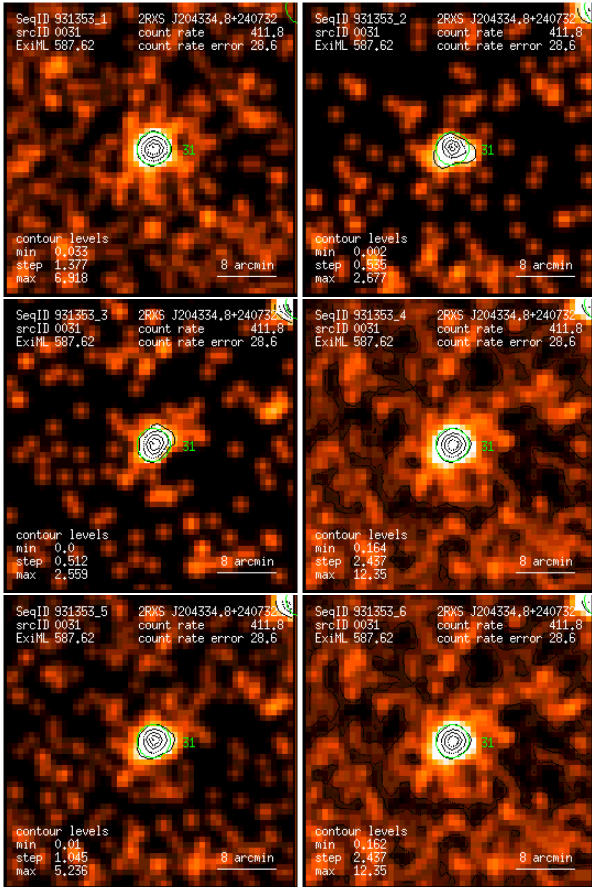
Figure 31: RASS 931353: detection 0031: band rate images, Gaussian filter: (1) PSPC channels 11 – 41, (2) 52 – 90, (3) 91 – 201, (4) 11 – 235, (5) 52 – 201, (6) 11 – 201. Broad band rates in counts/ks. Band rate contour levels in counts/ks/arcmin 2 .
