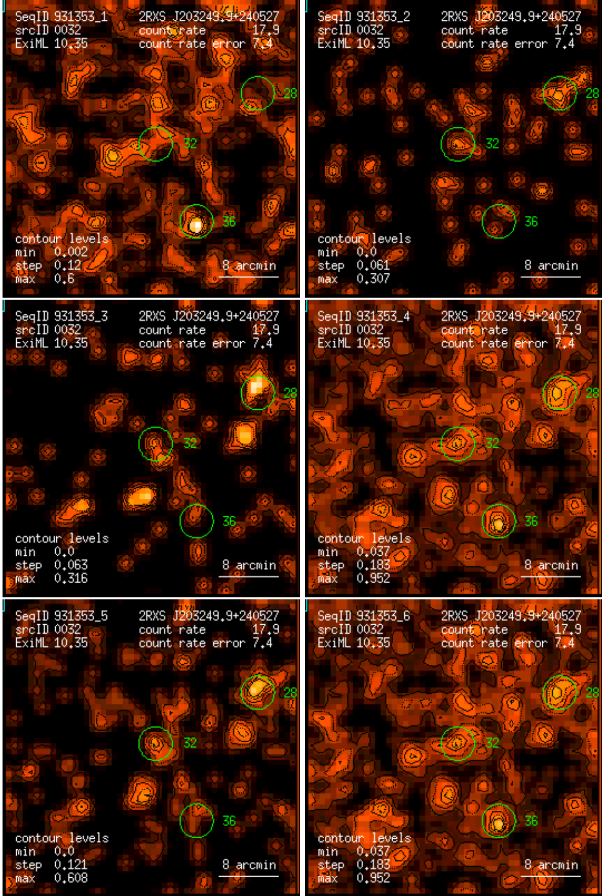
Figure 32: RASS 931353: detection 0032: band rate images, Gaussian filter: (1) PSPC channels 11 – 41, (2) 52 – 90, (3) 91 – 201, (4) 11 – 235, (5) 52 – 201, (6) 11 – 201. Broad band rates in counts/ks. Band rate contour levels in counts/ks/arcmin 2 .
