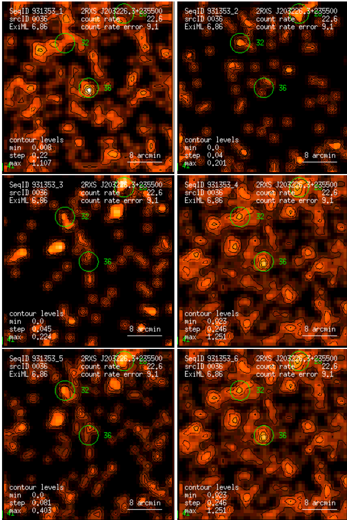
Figure 36: RASS 931353: detection 0036: band rate images, Gaussian filter: (1) PSPC channels 11 – 41, (2) 52 – 90, (3) 91 – 201, (4) 11 – 235, (5) 52 – 201, (6) 11 – 201. Broad band rates in counts/ks. Band rate contour levels in counts/ks/arcmin 2 .
