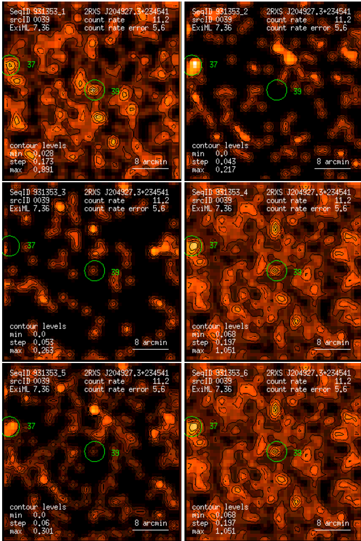
Figure 39: RASS 931353: detection 0039: band rate images, Gaussian filter: (1) PSPC channels 11 – 41, (2) 52 – 90, (3) 91 – 201, (4) 11 – 235, (5) 52 – 201, (6) 11 – 201. Broad band rates in counts/ks. Band rate contour levels in counts/ks/arcmin 2 .
