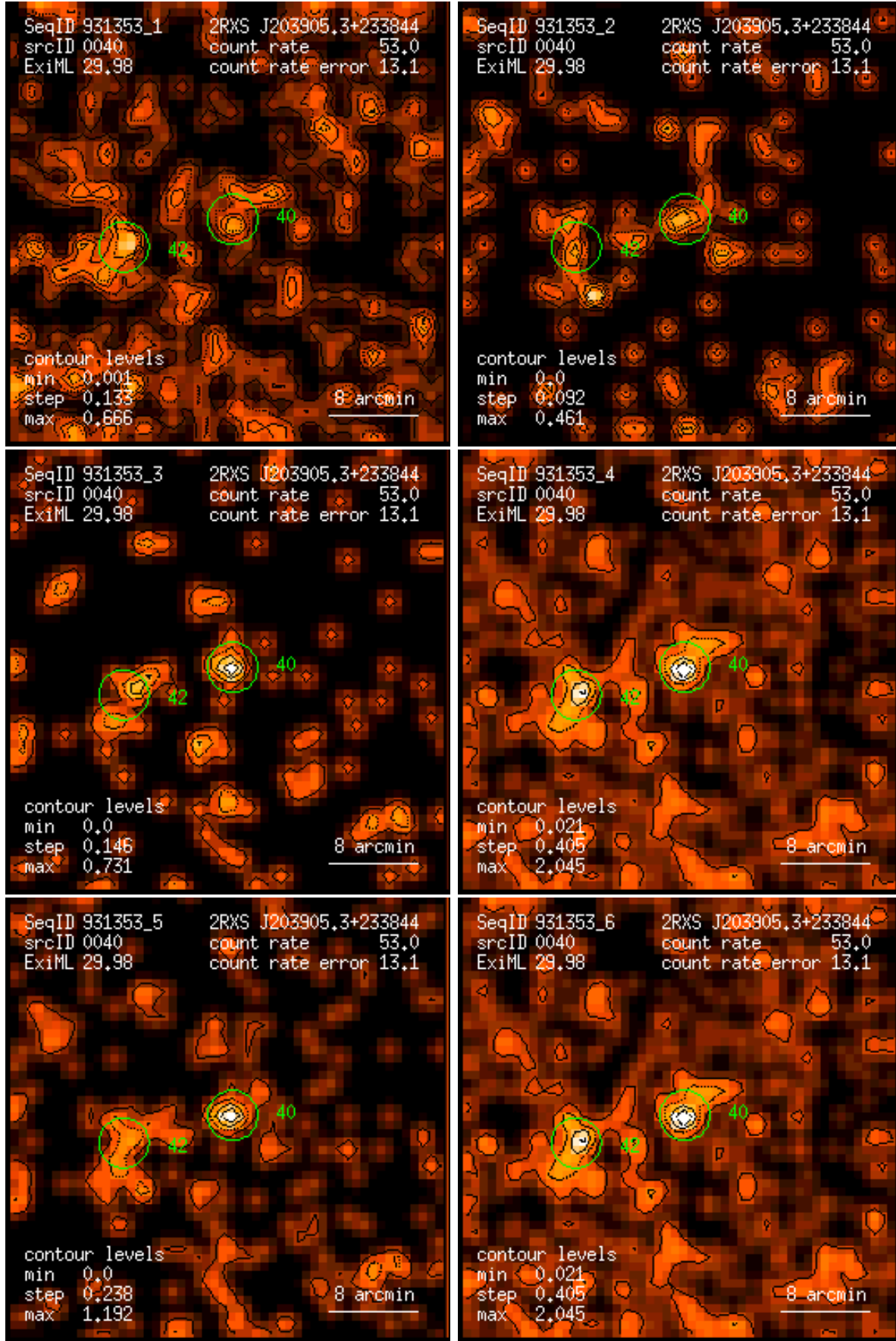
Figure 40: RASS 931353: detection 0040: band rate images, Gaussian filter: (1) PSPC channels 11 – 41, (2) 52 – 90, (3) 91 – 201, (4) 11 – 235, (5) 52 – 201, (6) 11 – 201. Broad band rates in counts/ks. Band rate contour levels in counts/ks/arcmin 2 .
