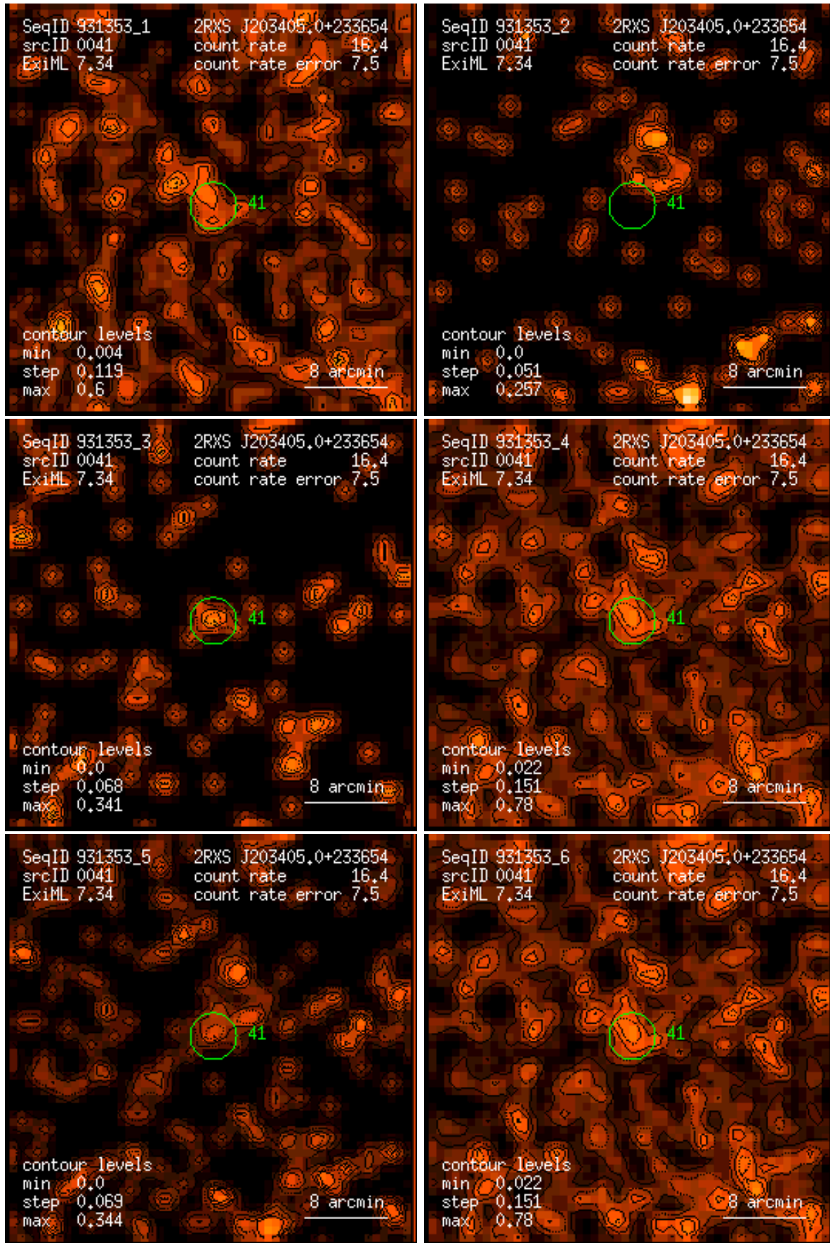
Figure 41: RASS 931353: detection 0041: band rate images, Gaussian filter: (1) PSPC channels 11 – 41, (2) 52 – 90, (3) 91 – 201, (4) 11 – 235, (5) 52 – 201, (6) 11 – 201. Broad band rates in counts/ks. Band rate contour levels in counts/ks/arcmin 2 .
