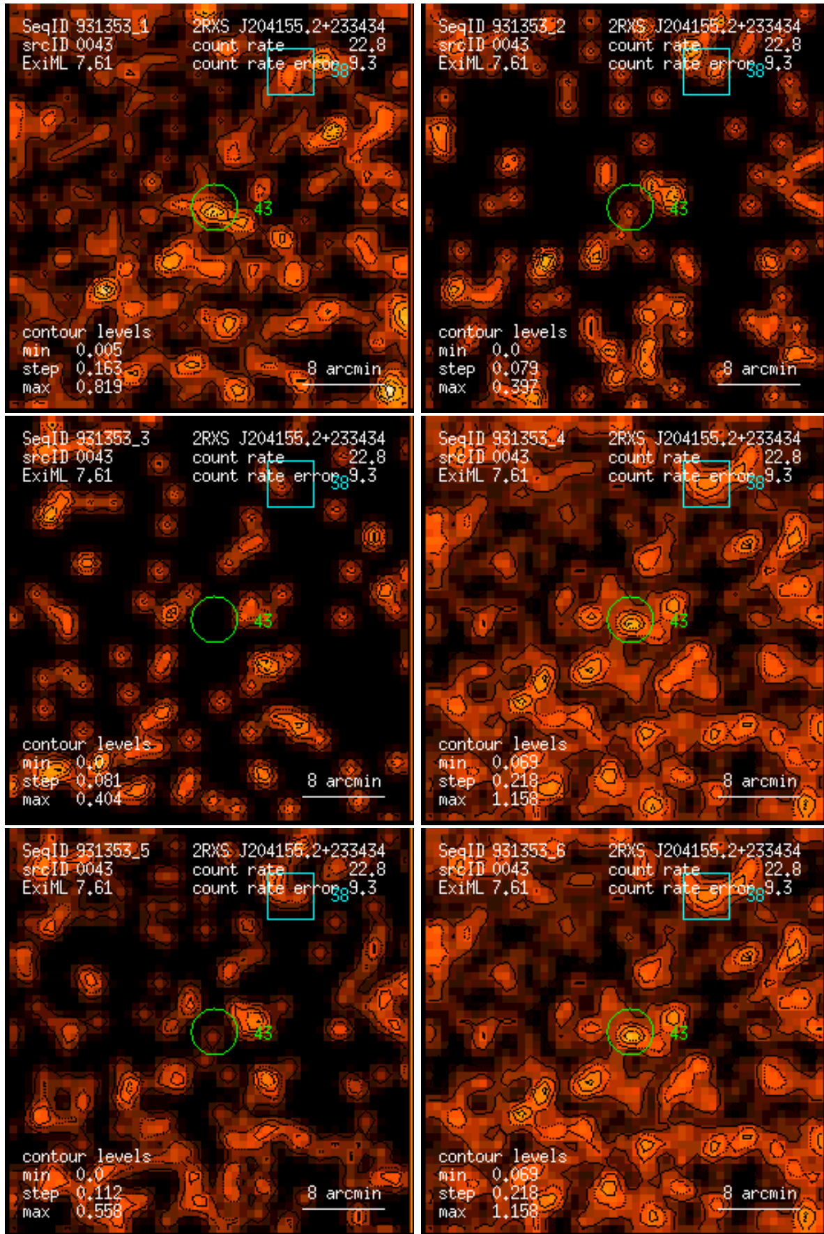
Figure 43: RASS 931353: detection 0043: band rate images, Gaussian filter: (1) PSPC channels 11 – 41, (2) 52 – 90, (3) 91 – 201, (4) 11 – 235, (5) 52 – 201, (6) 11 – 201. Broad band rates in counts/ks. Band rate contour levels in counts/ks/arcmin 2 .
