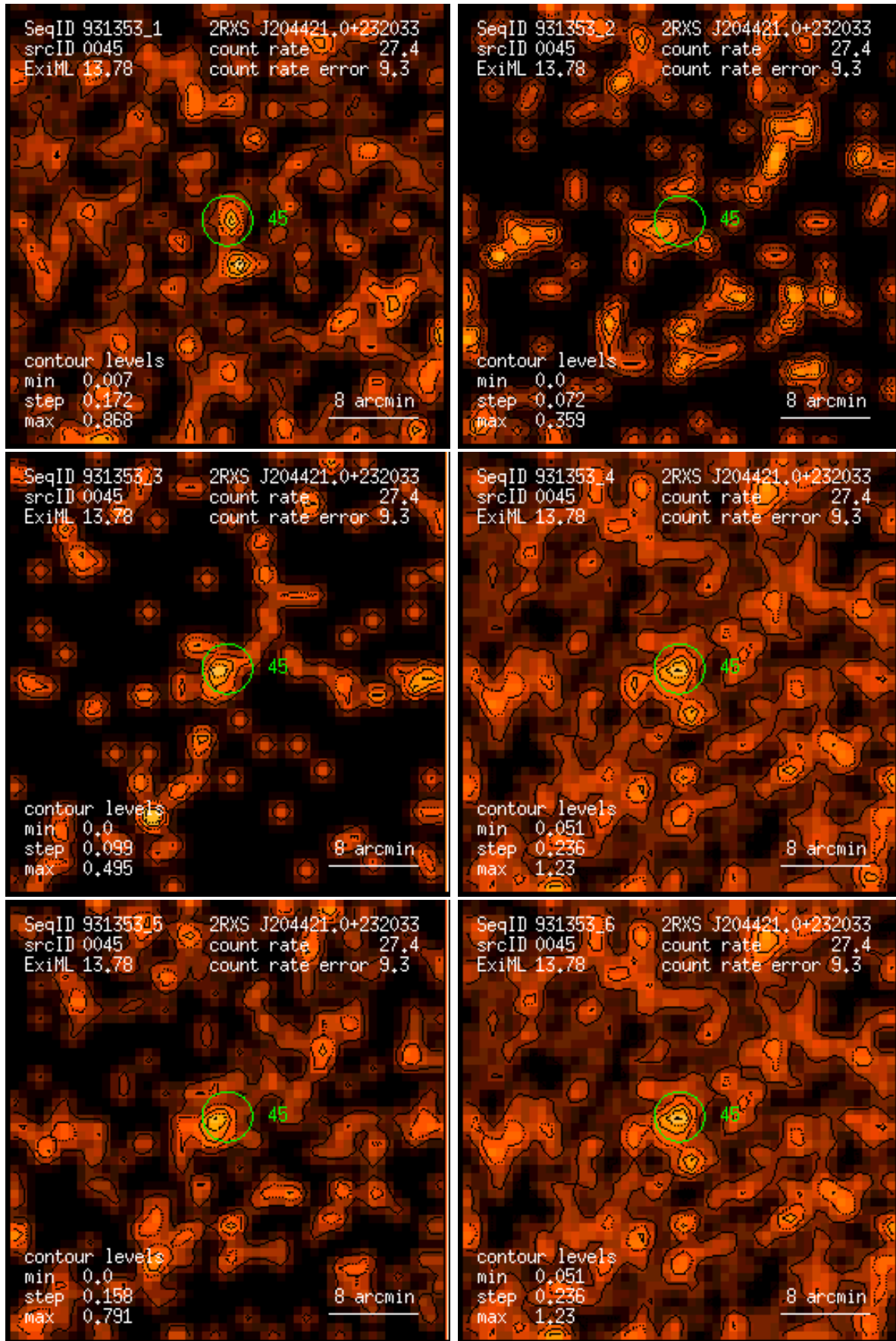
Figure 45: RASS 931353: detection 0045: band rate images, Gaussian filter: (1) PSPC channels 11 – 41, (2) 52 – 90, (3) 91 – 201, (4) 11 – 235, (5) 52 – 201, (6) 11 – 201. Broad band rates in counts/ks. Band rate contour levels in counts/ks/arcmin 2 .
