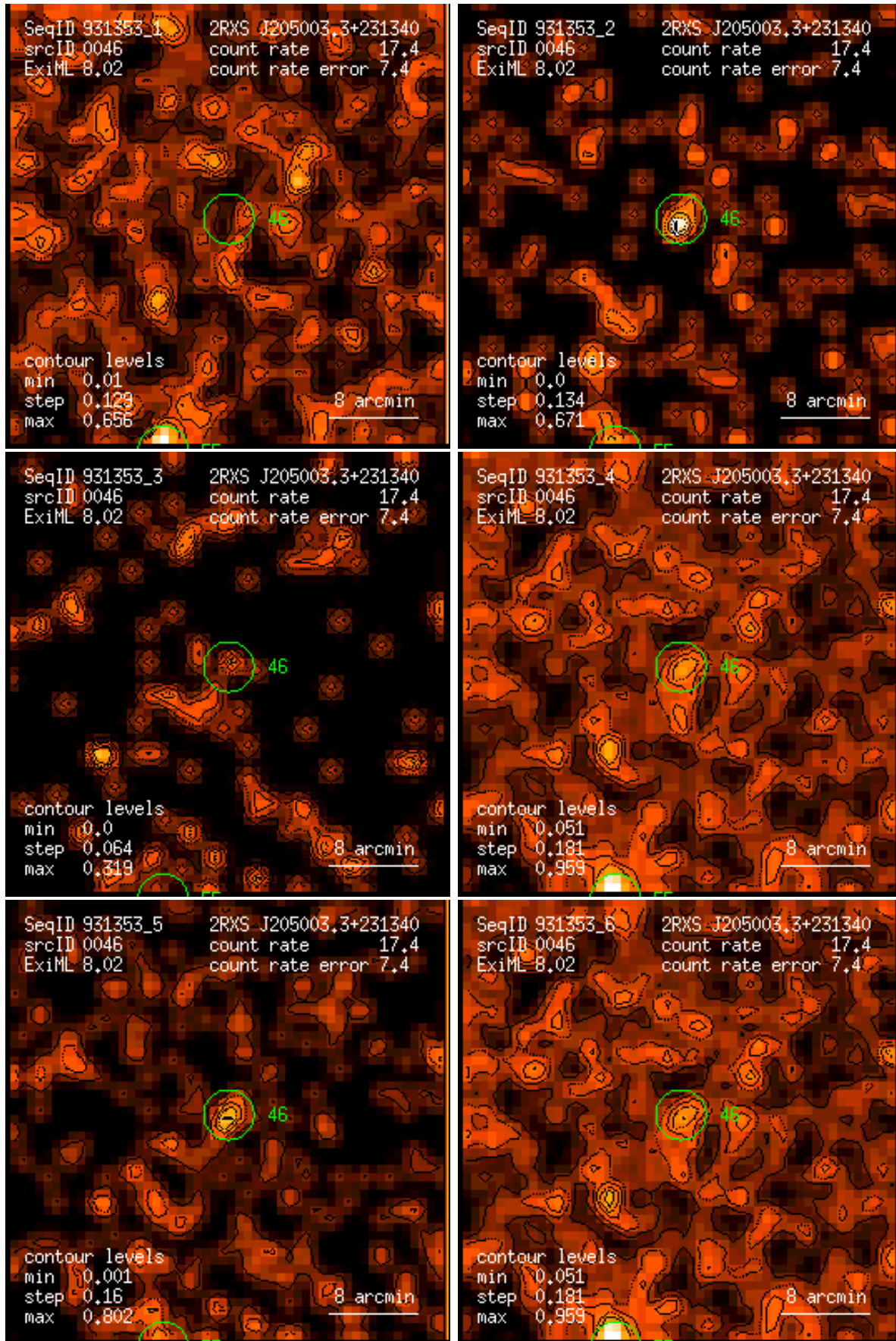
Figure 46: RASS 931353: detection 0046: band rate images, Gaussian filter: (1) PSPC channels 11 – 41, (2) 52 – 90, (3) 91 – 201, (4) 11 – 235, (5) 52 – 201, (6) 11 – 201. Broad band rates in counts/ks. Band rate contour levels in counts/ks/arcmin 2 .
