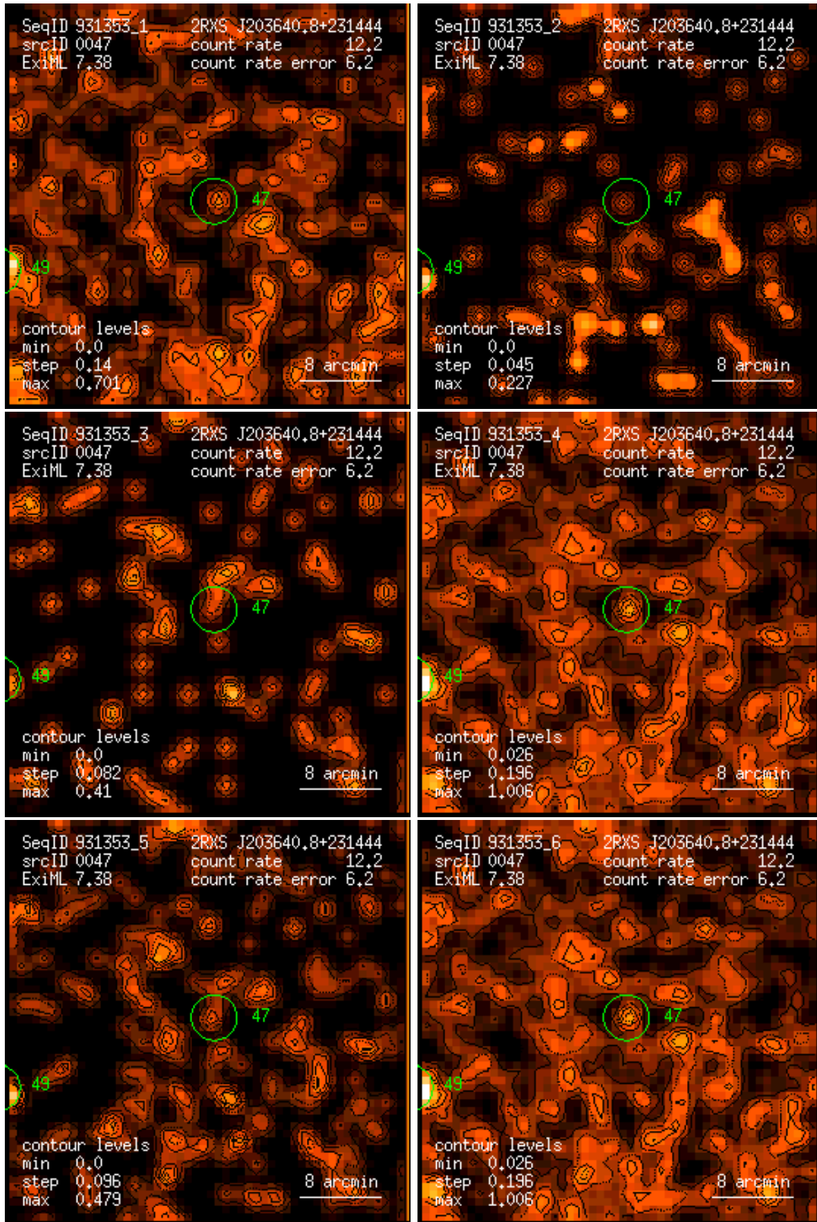
Figure 47: RASS 931353: detection 0047: band rate images, Gaussian filter: (1) PSPC channels 11 – 41, (2) 52 – 90, (3) 91 – 201, (4) 11 – 235, (5) 52 – 201, (6) 11 – 201. Broad band rates in counts/ks. Band rate contour levels in counts/ks/arcmin 2 .
