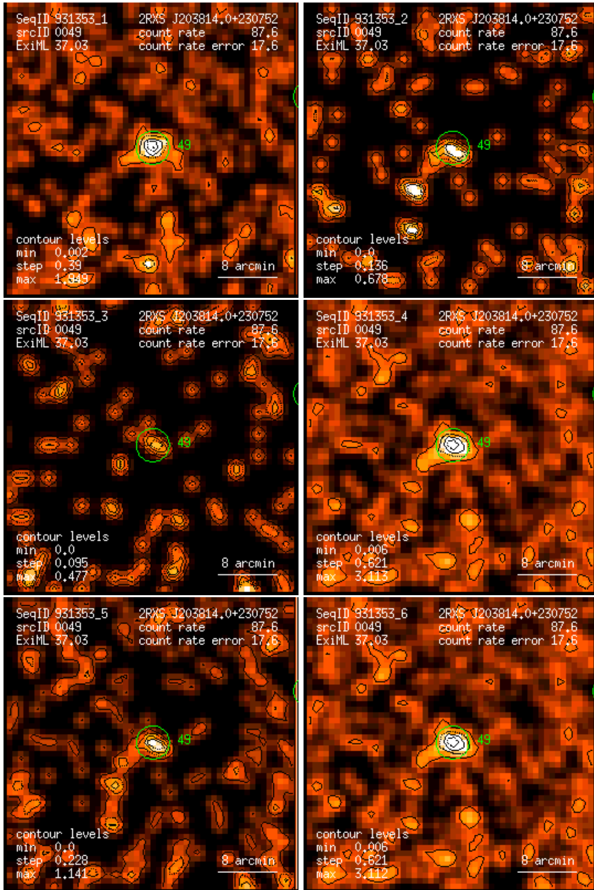
Figure 49: RASS 931353: detection 0049: band rate images, Gaussian filter: (1) PSPC channels 11 – 41, (2) 52 – 90, (3) 91 – 201, (4) 11 – 235, (5) 52 – 201, (6) 11 – 201. Broad band rates in counts/ks. Band rate contour levels in counts/ks/arcmin 2 .
