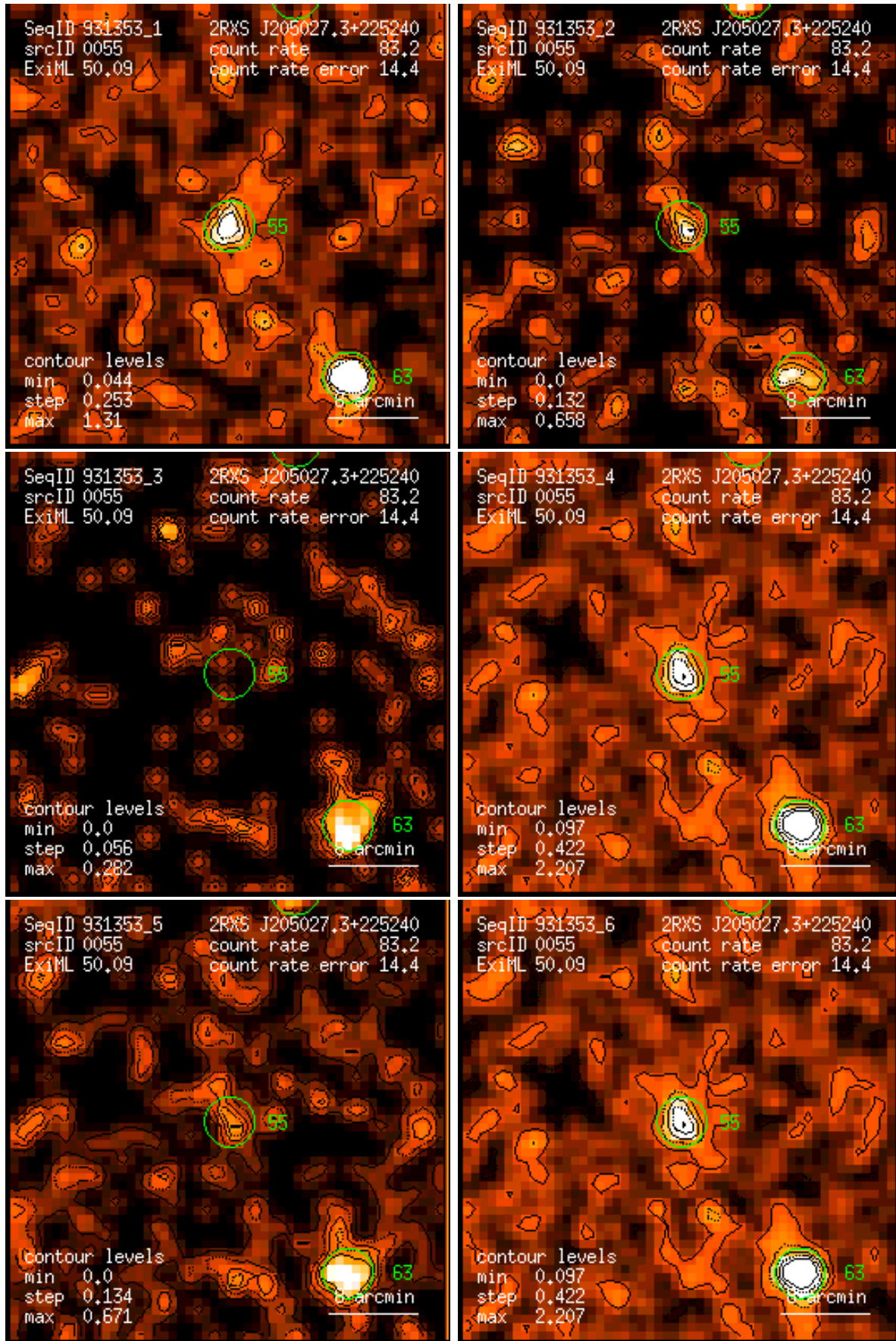
Figure 55: RASS 931353: detection 0055: band rate images, Gaussian filter: (1) PSPC channels 11 – 41, (2) 52 – 90, (3) 91 – 201, (4) 11 – 235, (5) 52 – 201, (6) 11 – 201. Broad band rates in counts/ks. Band rate contour levels in counts/ks/arcmin 2 .
