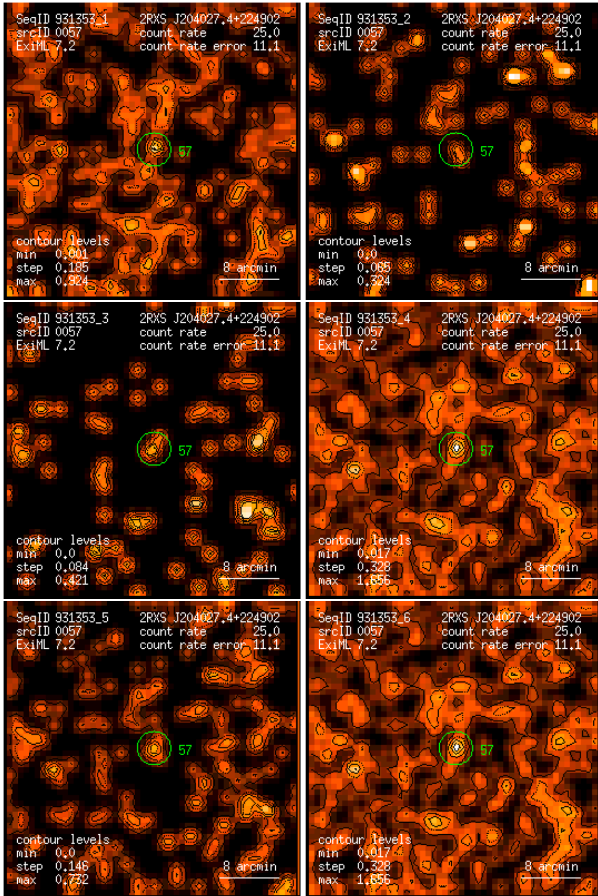
Figure 57: RASS 931353: detection 0057: band rate images, Gaussian filter: (1) PSPC channels 11 – 41, (2) 52 – 90, (3) 91 – 201, (4) 11 – 235, (5) 52 – 201, (6) 11 – 201. Broad band rates in counts/ks. Band rate contour levels in counts/ks/arcmin 2 .
