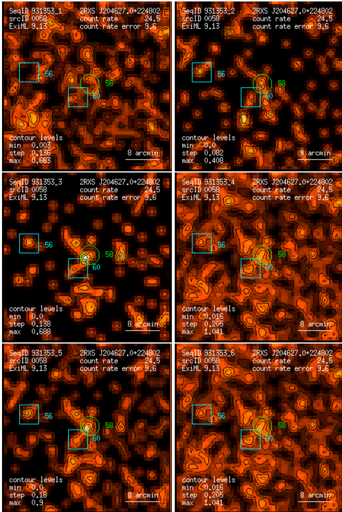
Figure 58: RASS 931353: detection 0058: band rate images, Gaussian filter: (1) PSPC channels 11 – 41, (2) 52 – 90, (3) 91 – 201, (4) 11 – 235, (5) 52 – 201, (6) 11 – 201. Broad band rates in counts/ks. Band rate contour levels in counts/ks/arcmin 2 .
