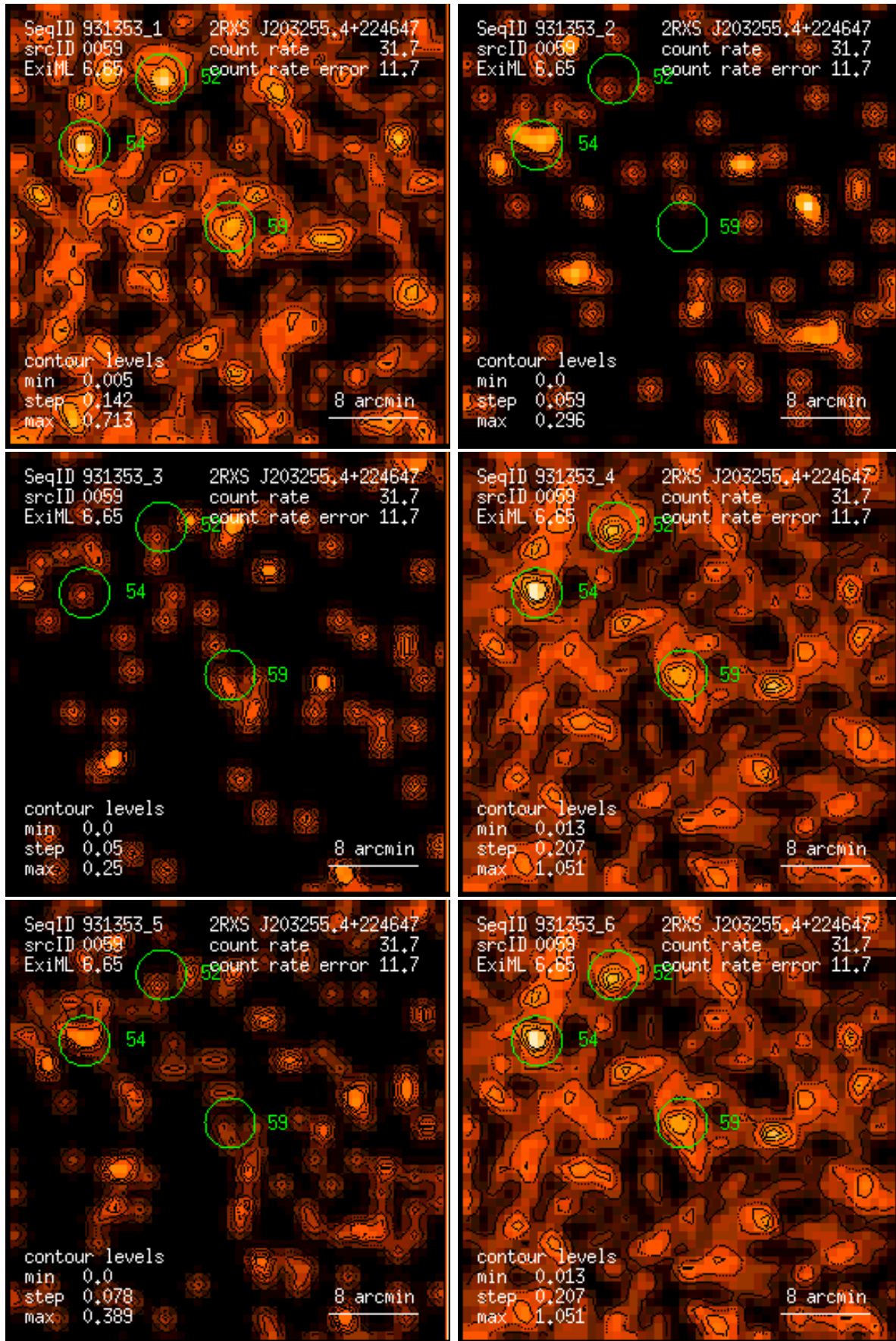
Figure 59: RASS 931353: detection 0059: band rate images, Gaussian filter: (1) PSPC channels 11 – 41, (2) 52 – 90, (3) 91 – 201, (4) 11 – 235, (5) 52 – 201, (6) 11 – 201. Broad band rates in counts/ks. Band rate contour levels in counts/ks/arcmin 2 .
