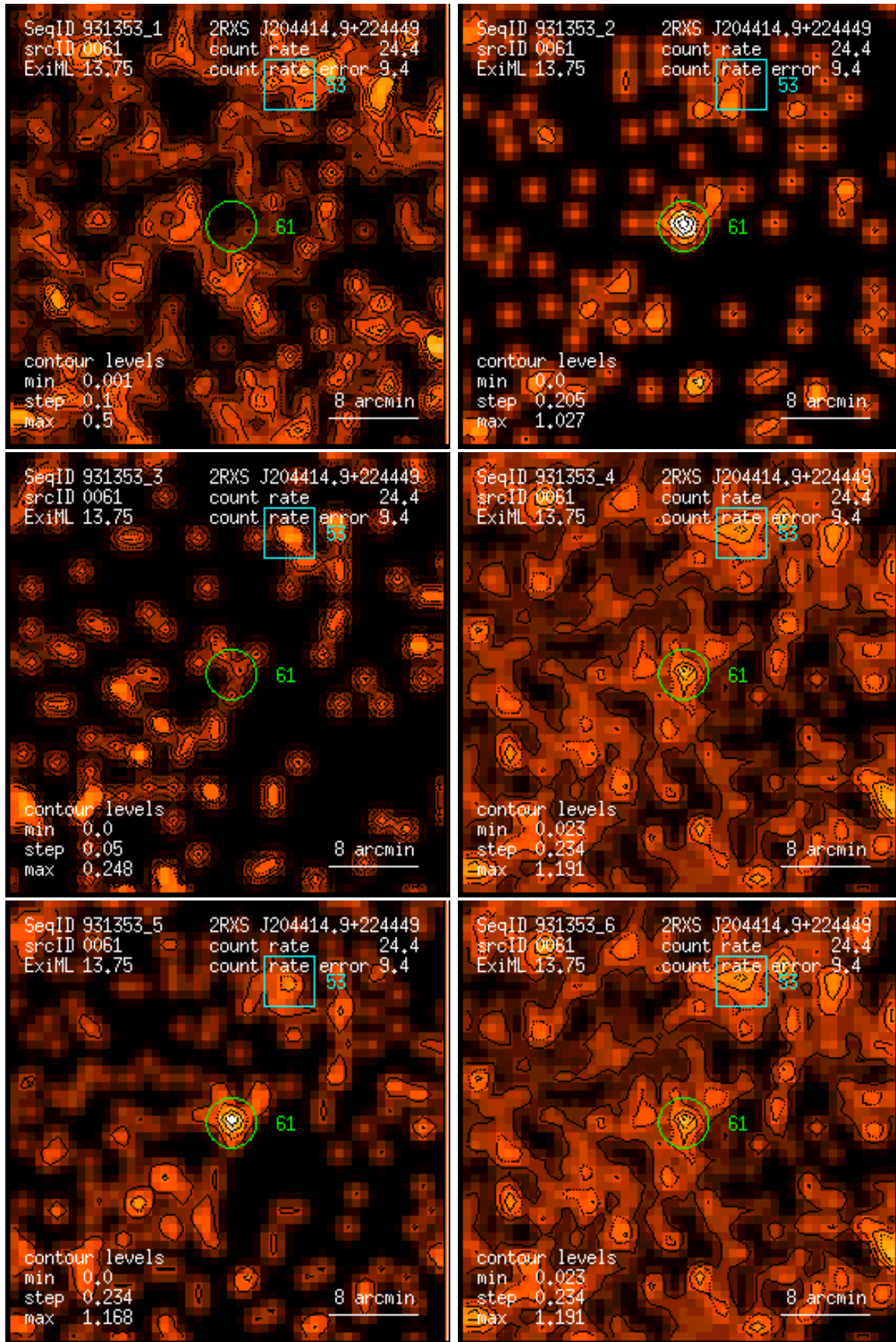
Figure 61: RASS 931353: detection 0061: band rate images, Gaussian filter: (1) PSPC channels 11 – 41, (2) 52 – 90, (3) 91 – 201, (4) 11 – 235, (5) 52 – 201, (6) 11 – 201. Broad band rates in counts/ks. Band rate contour levels in counts/ks/arcmin 2 .
