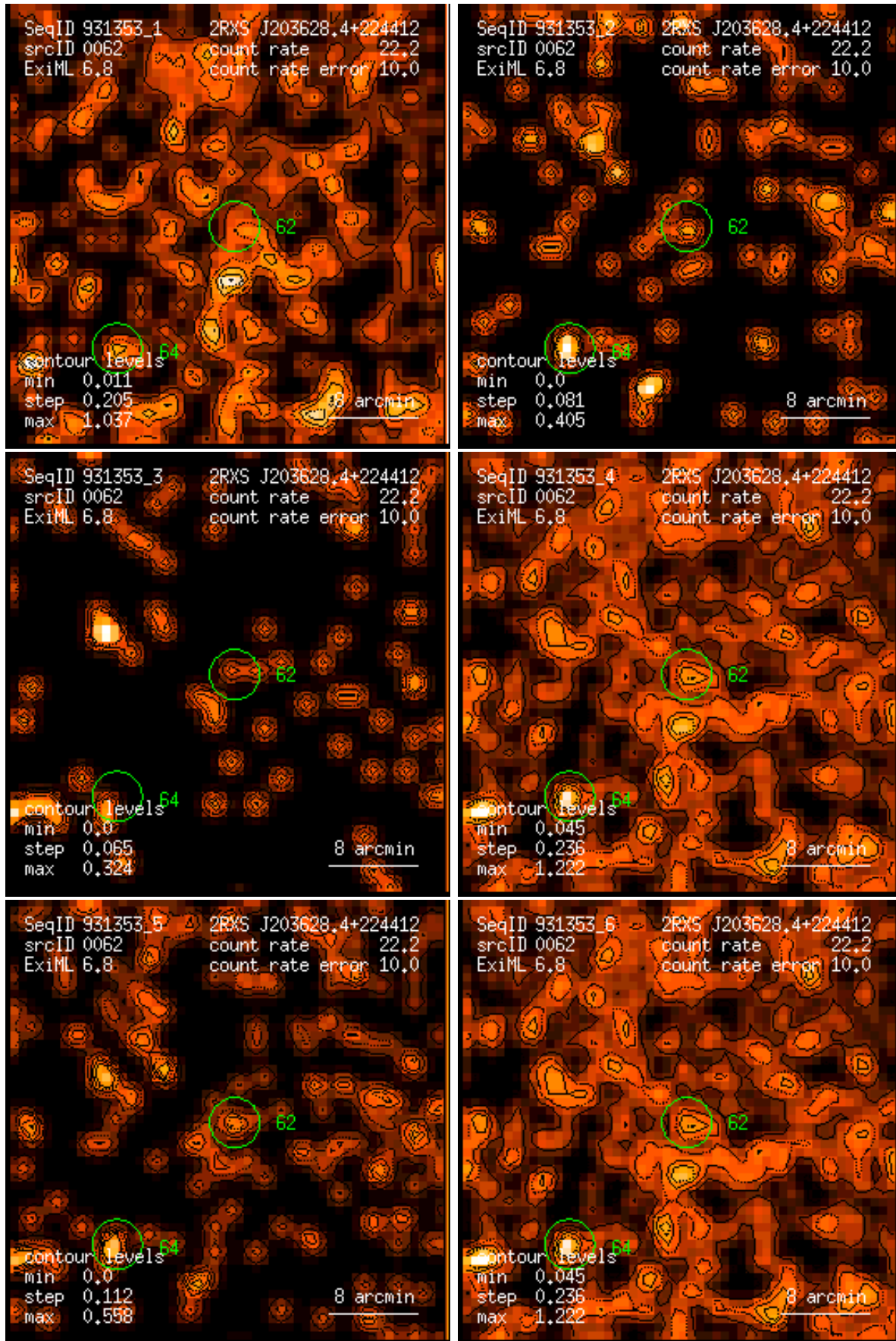
Figure 62: RASS 931353: detection 0062: band rate images, Gaussian filter: (1) PSPC channels 11 – 41, (2) 52 – 90, (3) 91 – 201, (4) 11 – 235, (5) 52 – 201, (6) 11 – 201. Broad band rates in counts/ks. Band rate contour levels in counts/ks/arcmin 2 .
