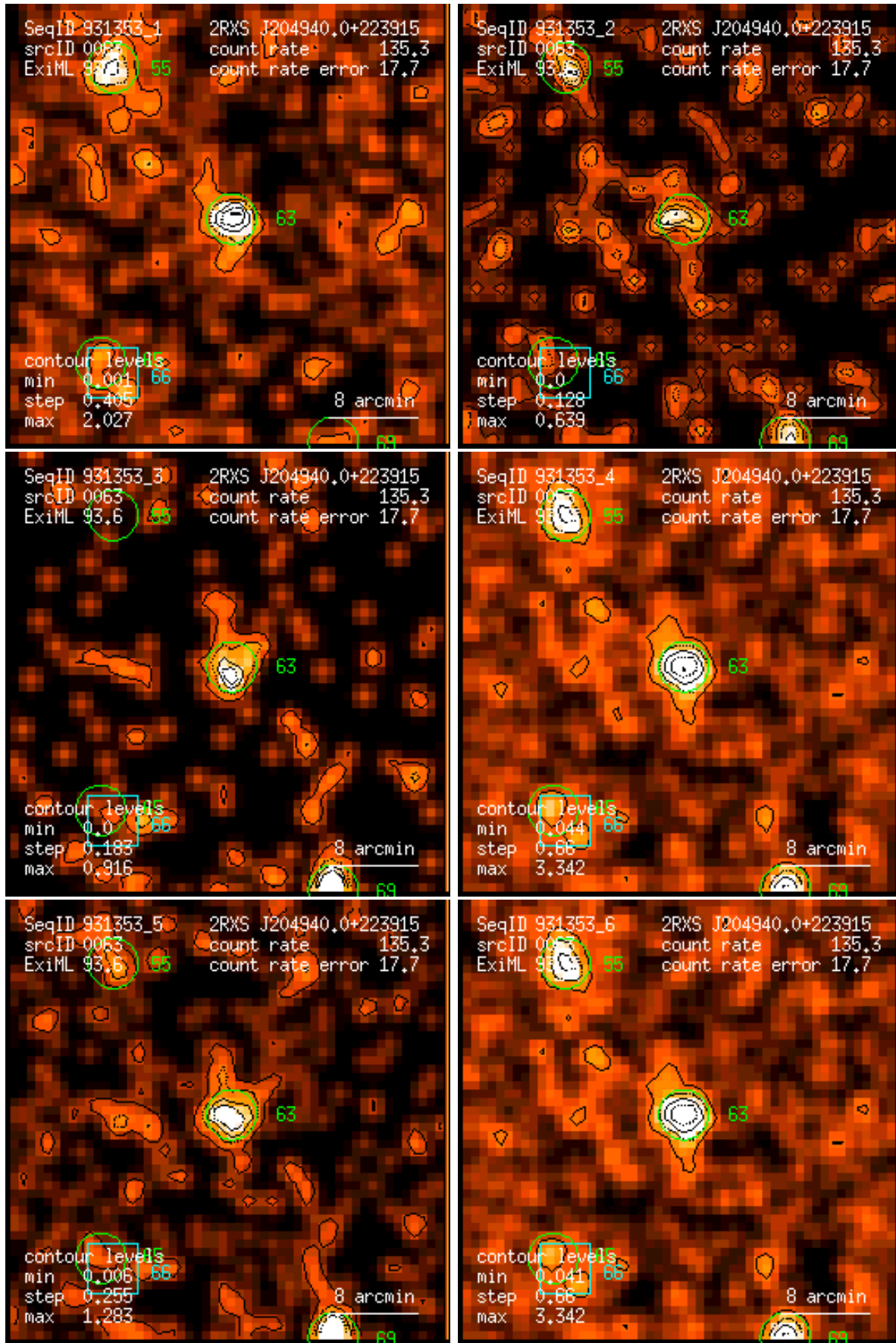
Figure 63: RASS 931353: detection 0063: band rate images, Gaussian filter: (1) PSPC channels 11 – 41, (2) 52 – 90, (3) 91 – 201, (4) 11 – 235, (5) 52 – 201, (6) 11 – 201. Broad band rates in counts/ks. Band rate contour levels in counts/ks/arcmin 2 .
