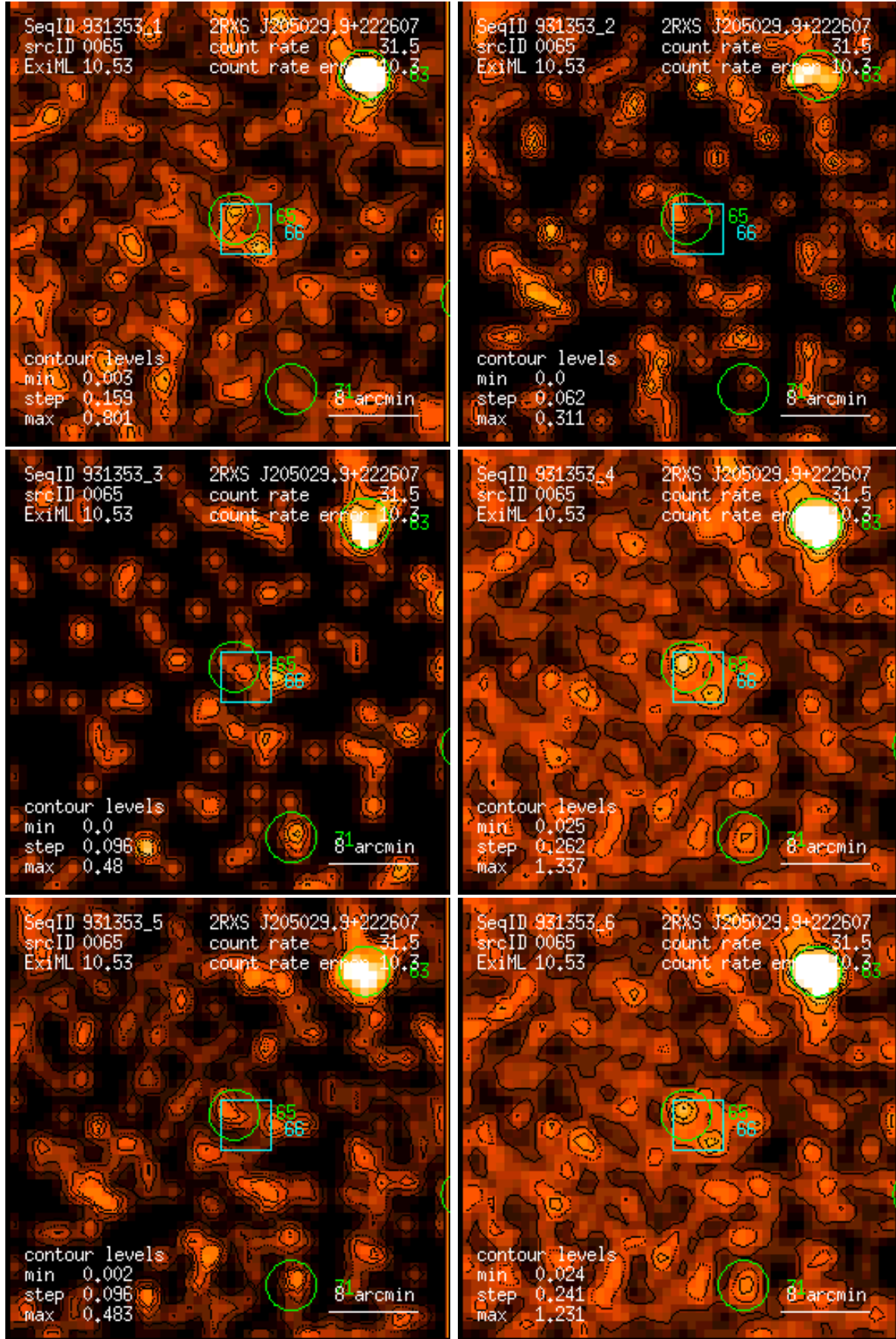
Figure 65: RASS 931353: detection 0065: band rate images, Gaussian filter: (1) PSPC channels 11 – 41, (2) 52 – 90, (3) 91 – 201, (4) 11 – 235, (5) 52 – 201, (6) 11 – 201. Broad band rates in counts/ks. Band rate contour levels in counts/ks/arcmin 2 .
