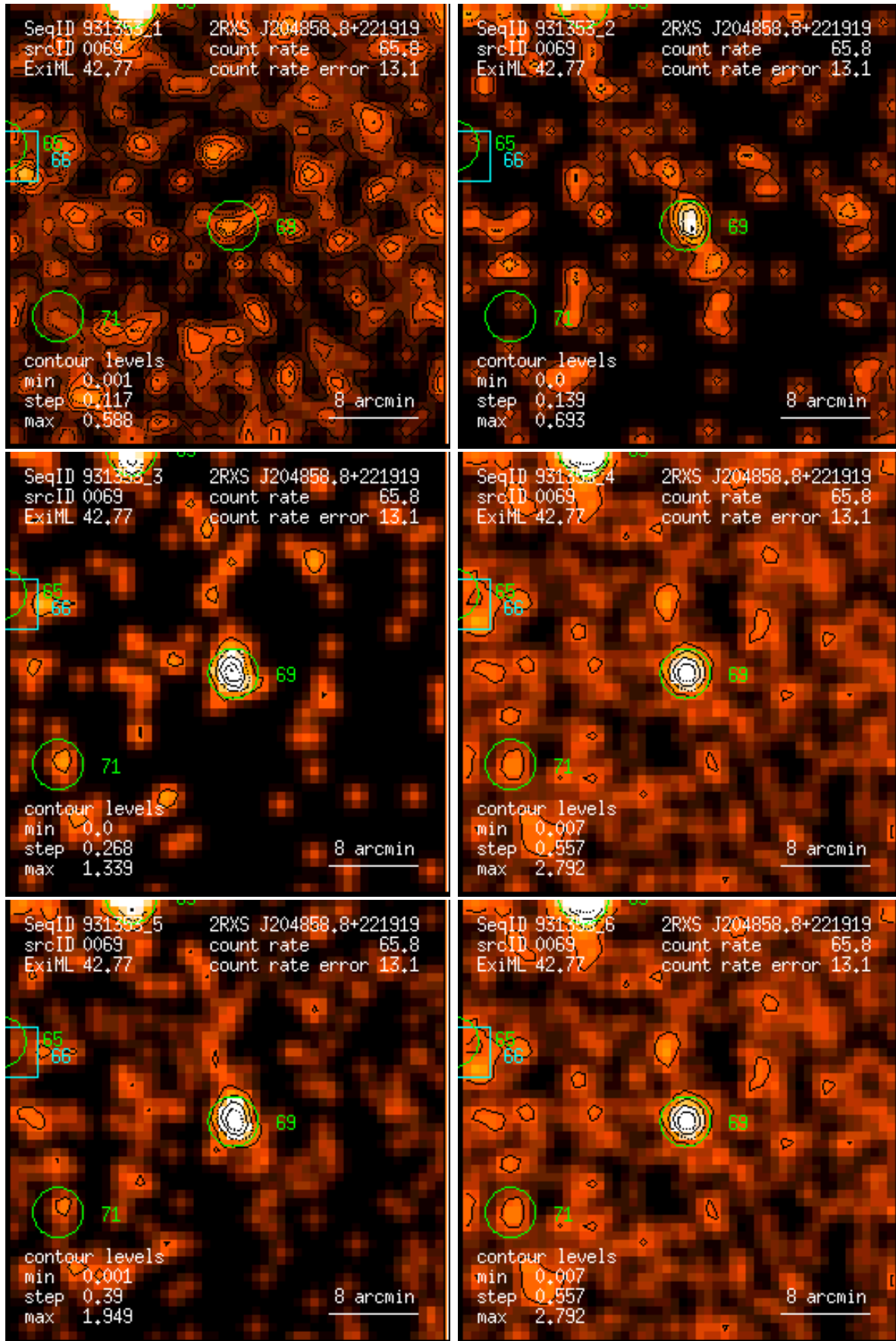
Figure 69: RASS 931353: detection 0069: band rate images, Gaussian filter: (1) PSPC channels 11 – 41, (2) 52 – 90, (3) 91 – 201, (4) 11 – 235, (5) 52 – 201, (6) 11 – 201. Broad band rates in counts/ks. Band rate contour levels in counts/ks/arcmin 2 .
