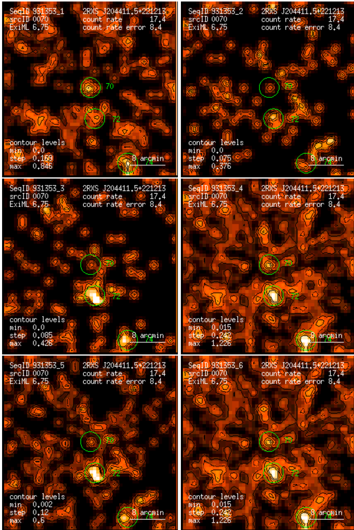
Figure 70: RASS 931353: detection 0070: band rate images, Gaussian filter: (1) PSPC channels 11 – 41, (2) 52 – 90, (3) 91 – 201, (4) 11 – 235, (5) 52 – 201, (6) 11 – 201. Broad band rates in counts/ks. Band rate contour levels in counts/ks/arcmin 2 .
