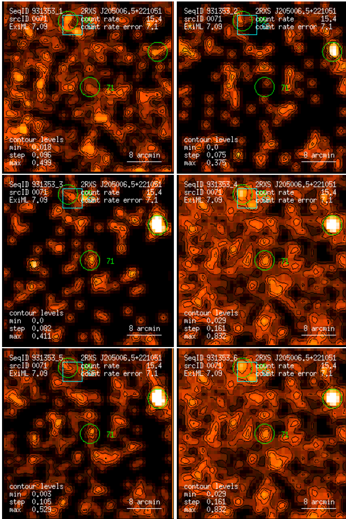
Figure 71: RASS 931353: detection 0071: band rate images, Gaussian filter: (1) PSPC channels 11 – 41, (2) 52 – 90, (3) 91 – 201, (4) 11 – 235, (5) 52 – 201, (6) 11 – 201. Broad band rates in counts/ks. Band rate contour levels in counts/ks/arcmin 2 .
