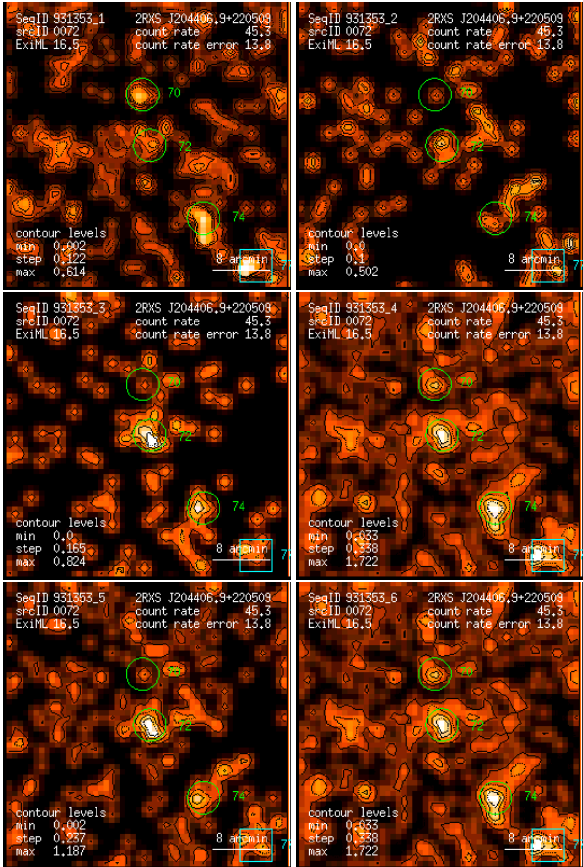
Figure 72: RASS 931353: detection 0072: band rate images, Gaussian filter: (1) PSPC channels 11 – 41, (2) 52 – 90, (3) 91 – 201, (4) 11 – 235, (5) 52 – 201, (6) 11 – 201. Broad band rates in counts/ks. Band rate contour levels in counts/ks/arcmin 2 .
