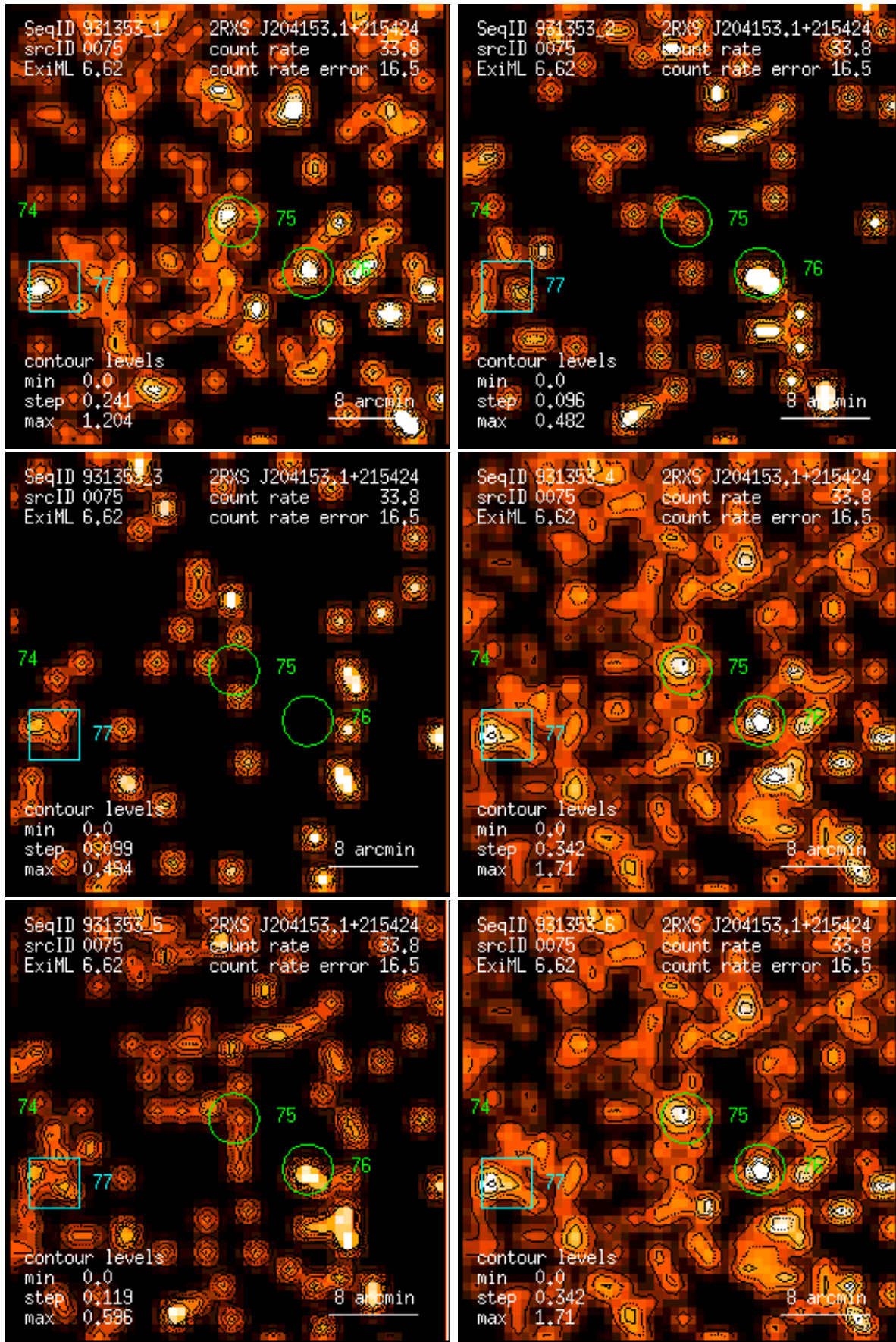
Figure 75: RASS 931353: detection 0075: band rate images, Gaussian filter: (1) PSPC channels 11 – 41, (2) 52 – 90, (3) 91 – 201, (4) 11 – 235, (5) 52 – 201, (6) 11 – 201. Broad band rates in counts/ks. Band rate contour levels in counts/ks/arcmin 2 .
