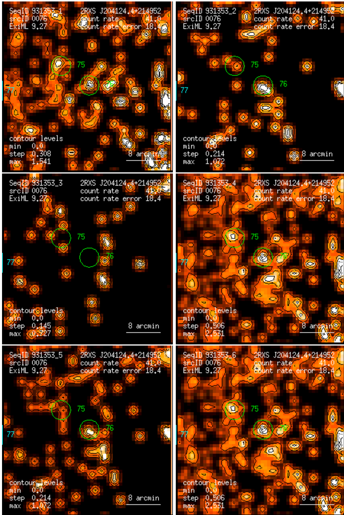
Figure 76: RASS 931353: detection 0076: band rate images, Gaussian filter: (1) PSPC channels 11 – 41, (2) 52 – 90, (3) 91 – 201, (4) 11 – 235, (5) 52 – 201, (6) 11 – 201. Broad band rates in counts/ks. Band rate contour levels in counts/ks/arcmin 2 .
