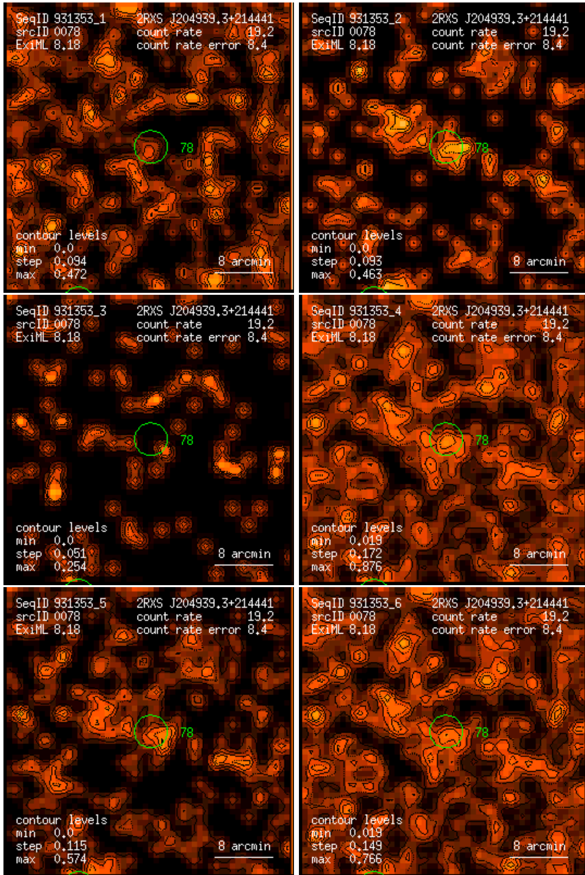
Figure 78: RASS 931353: detection 0078: band rate images, Gaussian filter: (1) PSPC channels 11 – 41, (2) 52 – 90, (3) 91 – 201, (4) 11 – 235, (5) 52 – 201, (6) 11 – 201. Broad band rates in counts/ks. Band rate contour levels in counts/ks/arcmin 2 .
