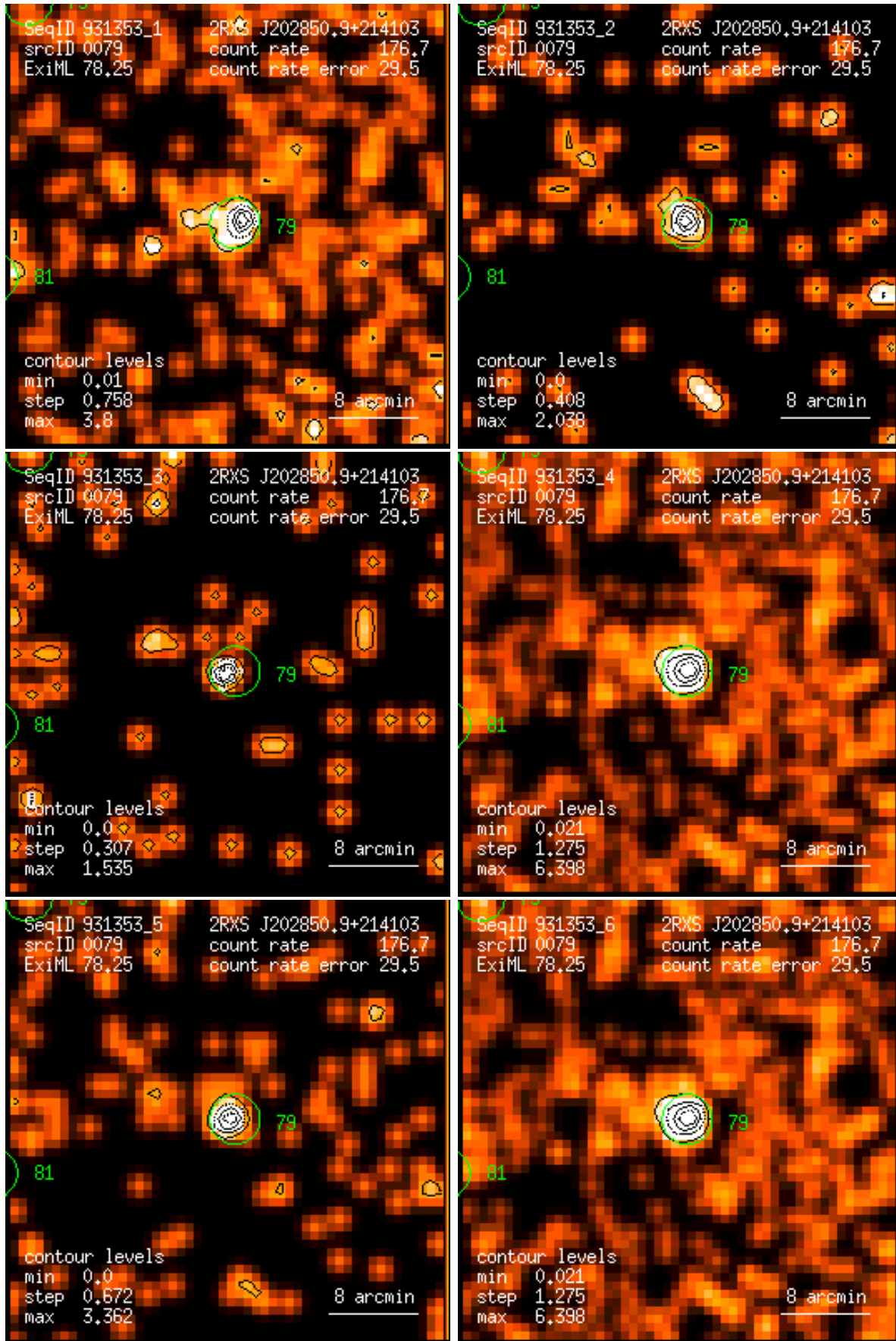
Figure 79: RASS 931353: detection 0079: band rate images, Gaussian filter: (1) PSPC channels 11 – 41, (2) 52 – 90, (3) 91 – 201, (4) 11 – 235, (5) 52 – 201, (6) 11 – 201. Broad band rates in counts/ks. Band rate contour levels in counts/ks/arcmin 2 .
