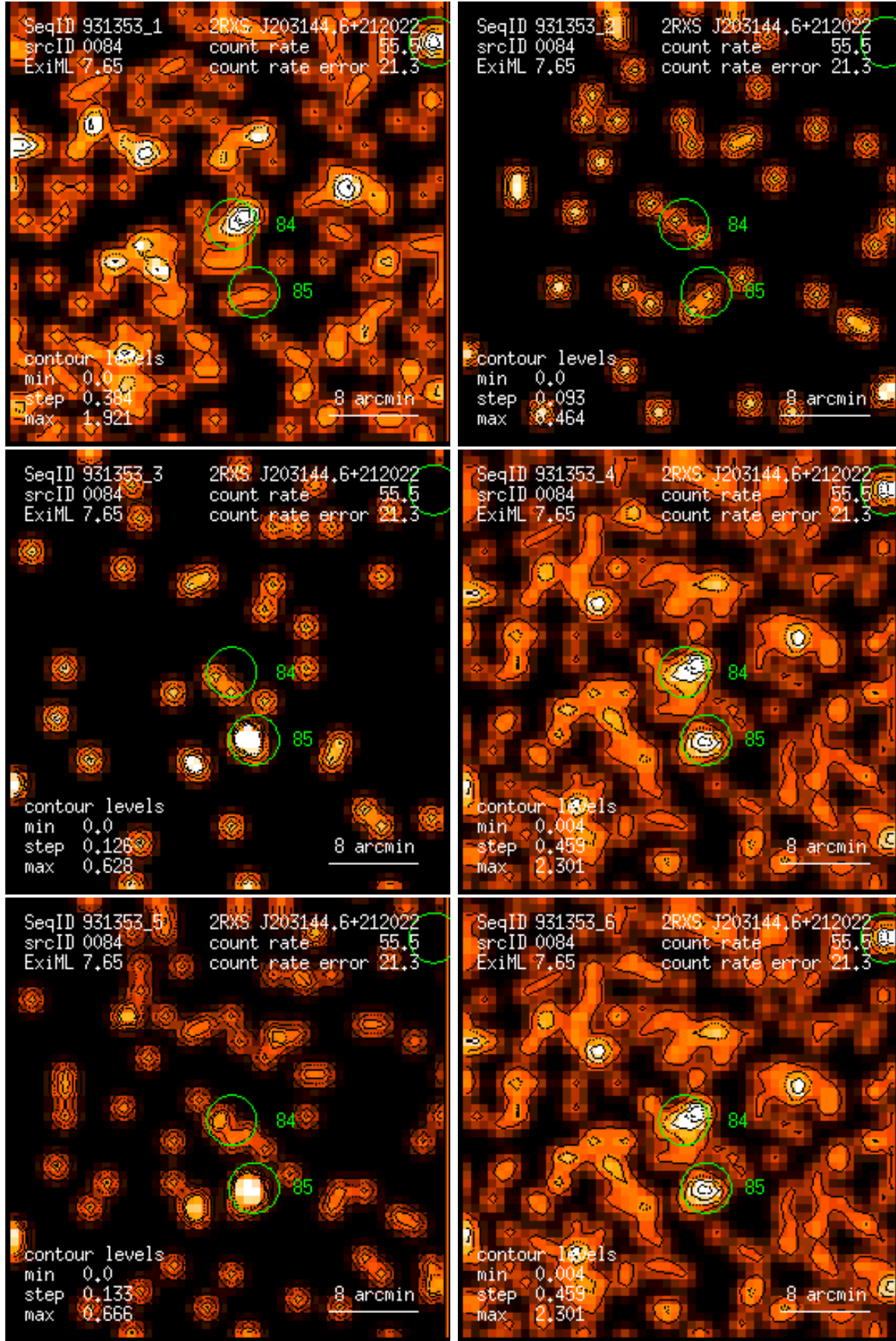
Figure 84: RASS 931353: detection 0084: band rate images, Gaussian filter: (1) PSPC channels 11 – 41, (2) 52 – 90, (3) 91 – 201, (4) 11 – 235, (5) 52 – 201, (6) 11 – 201. Broad band rates in counts/ks. Band rate contour levels in counts/ks/arcmin 2 .
