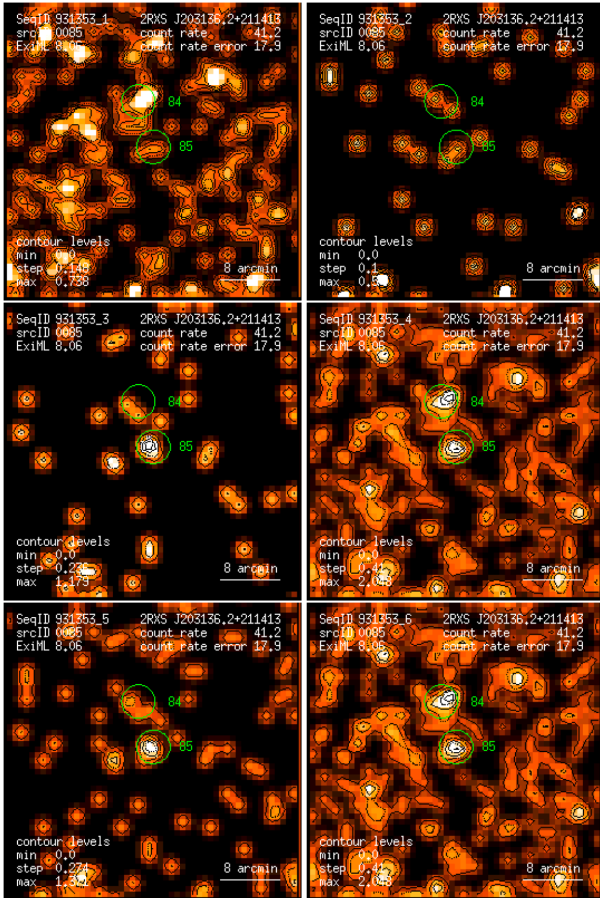
Figure 85: RASS 931353: detection 0085: band rate images, Gaussian filter: (1) PSPC channels 11 – 41, (2) 52 – 90, (3) 91 – 201, (4) 11 – 235, (5) 52 – 201, (6) 11 – 201. Broad band rates in counts/ks. Band rate contour levels in counts/ks/arcmin 2 .
