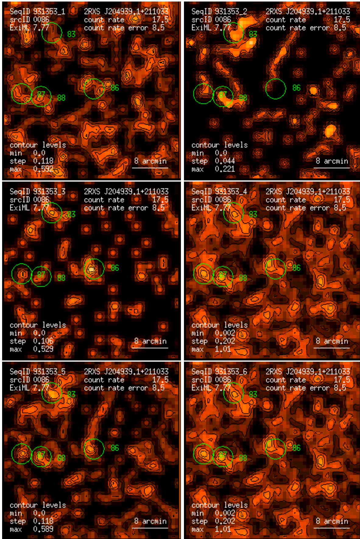
Figure 86: RASS 931353: detection 0086: band rate images, Gaussian filter: (1) PSPC channels 11 – 41, (2) 52 – 90, (3) 91 – 201, (4) 11 – 235, (5) 52 – 201, (6) 11 – 201. Broad band rates in counts/ks. Band rate contour levels in counts/ks/arcmin 2 .
