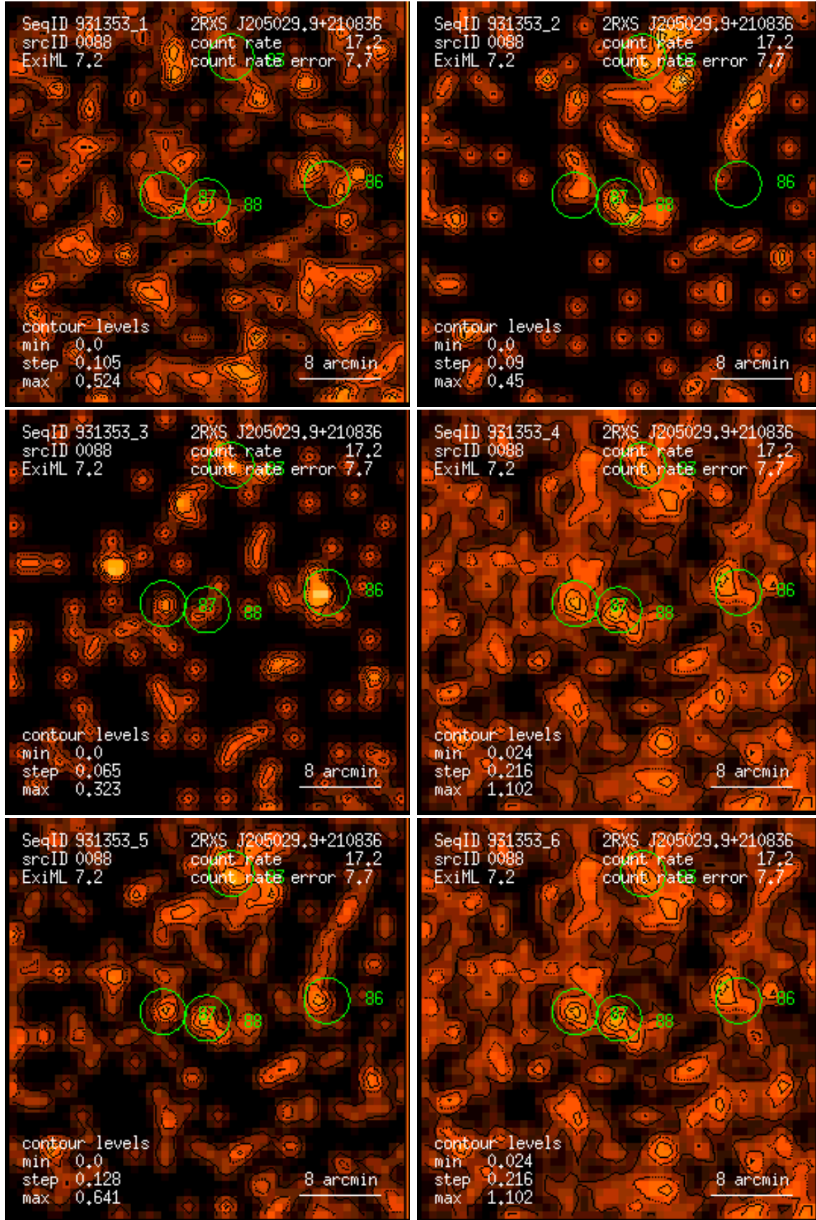
Figure 88: RASS 931353: detection 0088: band rate images, Gaussian filter: (1) PSPC channels 11 – 41, (2) 52 – 90, (3) 91 – 201, (4) 11 – 235, (5) 52 – 201, (6) 11 – 201. Broad band rates in counts/ks. Band rate contour levels in counts/ks/arcmin 2 .
