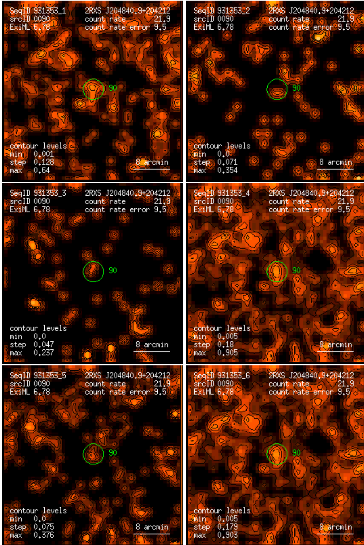
Figure 90: RASS 931353: detection 0090: band rate images, Gaussian filter: (1) PSPC channels 11 – 41, (2) 52 – 90, (3) 91 – 201, (4) 11 – 235, (5) 52 – 201, (6) 11 – 201. Broad band rates in counts/ks. Band rate contour levels in counts/ks/arcmin 2 .
