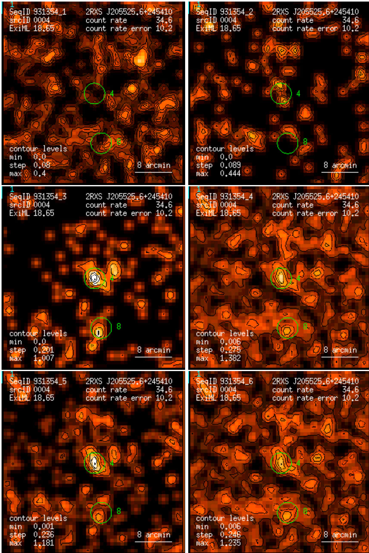
Figure 4: RASS 931354: detection 0004: band rate images, Gaussian filter: (1) PSPC channels 11 – 41, (2) 52 – 90, (3) 91 – 201, (4) 11 – 235, (5) 52 – 201, (6) 11 – 201. Broad band rates in counts/ks. Band rate contour levels in counts/ks/arcmin 2 .
