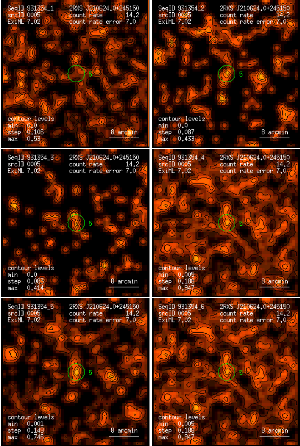
Figure 5: RASS 931354: detection 0005: band rate images, Gaussian filter: (1) PSPC channels 11 – 41, (2) 52 – 90, (3) 91 – 201, (4) 11 – 235, (5) 52 – 201, (6) 11 – 201. Broad band rates in counts/ks. Band rate contour levels in counts/ks/arcmin 2 .
