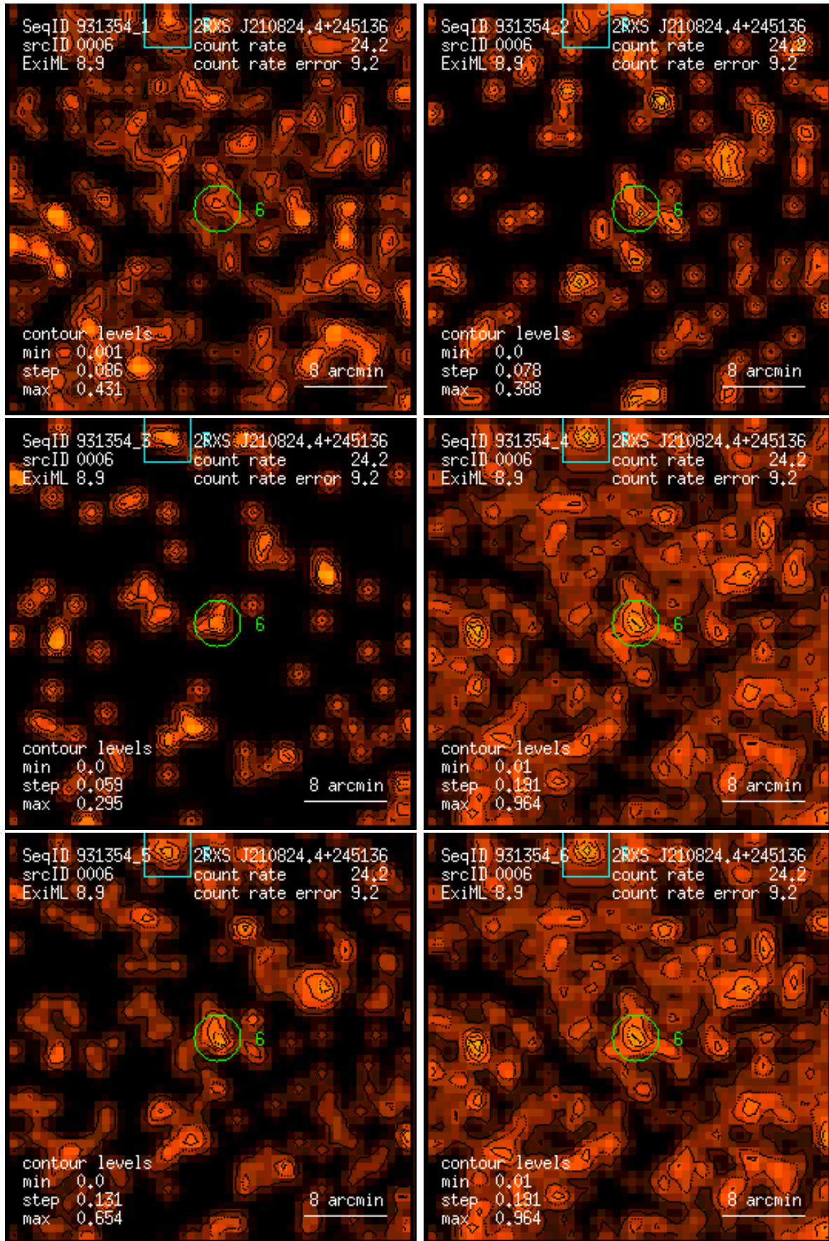
Figure 6: RASS 931354: detection 0006: band rate images, Gaussian filter: (1) PSPC channels 11 – 41, (2) 52 – 90, (3) 91 – 201, (4) 11 – 235, (5) 52 – 201, (6) 11 – 201. Broad band rates in counts/ks. Band rate contour levels in counts/ks/arcmin 2 .
