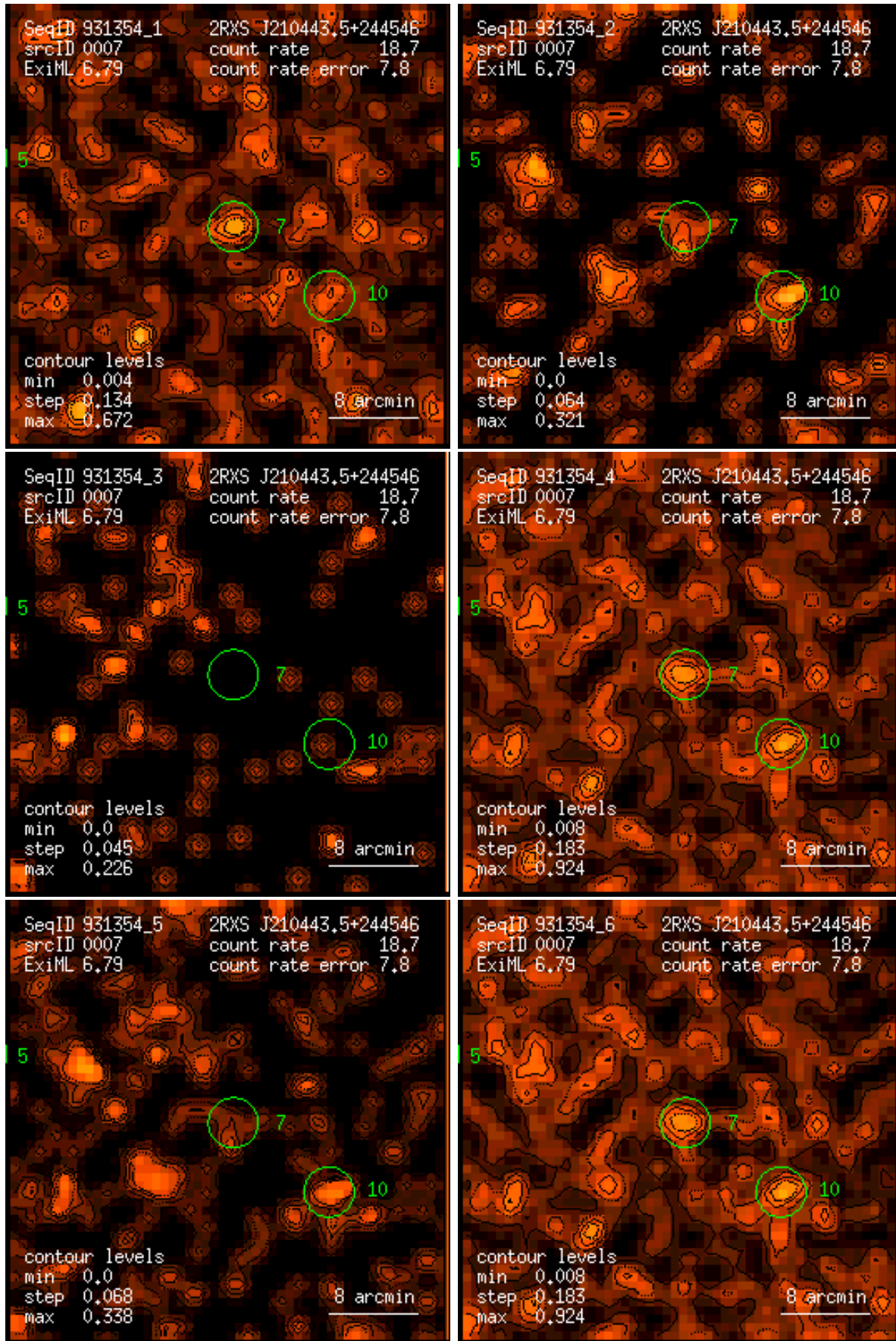
Figure 7: RASS 931354: detection 0007: band rate images, Gaussian filter: (1) PSPC channels 11 – 41, (2) 52 – 90, (3) 91 – 201, (4) 11 – 235, (5) 52 – 201, (6) 11 – 201. Broad band rates in counts/ks. Band rate contour levels in counts/ks/arcmin 2 .
