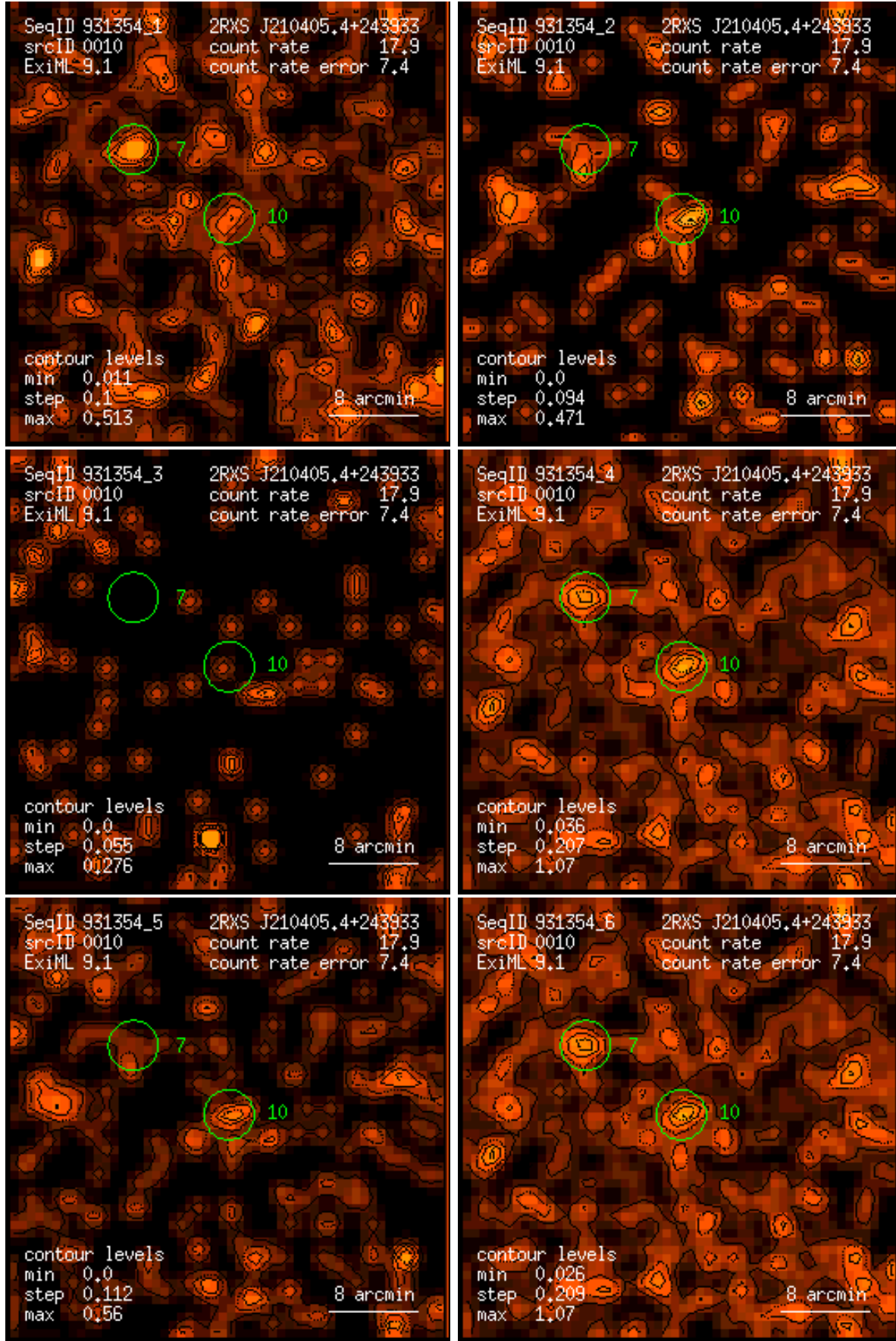
Figure 10: RASS 931354: detection 0010: band rate images, Gaussian filter: (1) PSPC channels 11 – 41, (2) 52 – 90, (3) 91 – 201, (4) 11 – 235, (5) 52 – 201, (6) 11 – 201. Broad band rates in counts/ks. Band rate contour levels in counts/ks/arcmin 2 .
