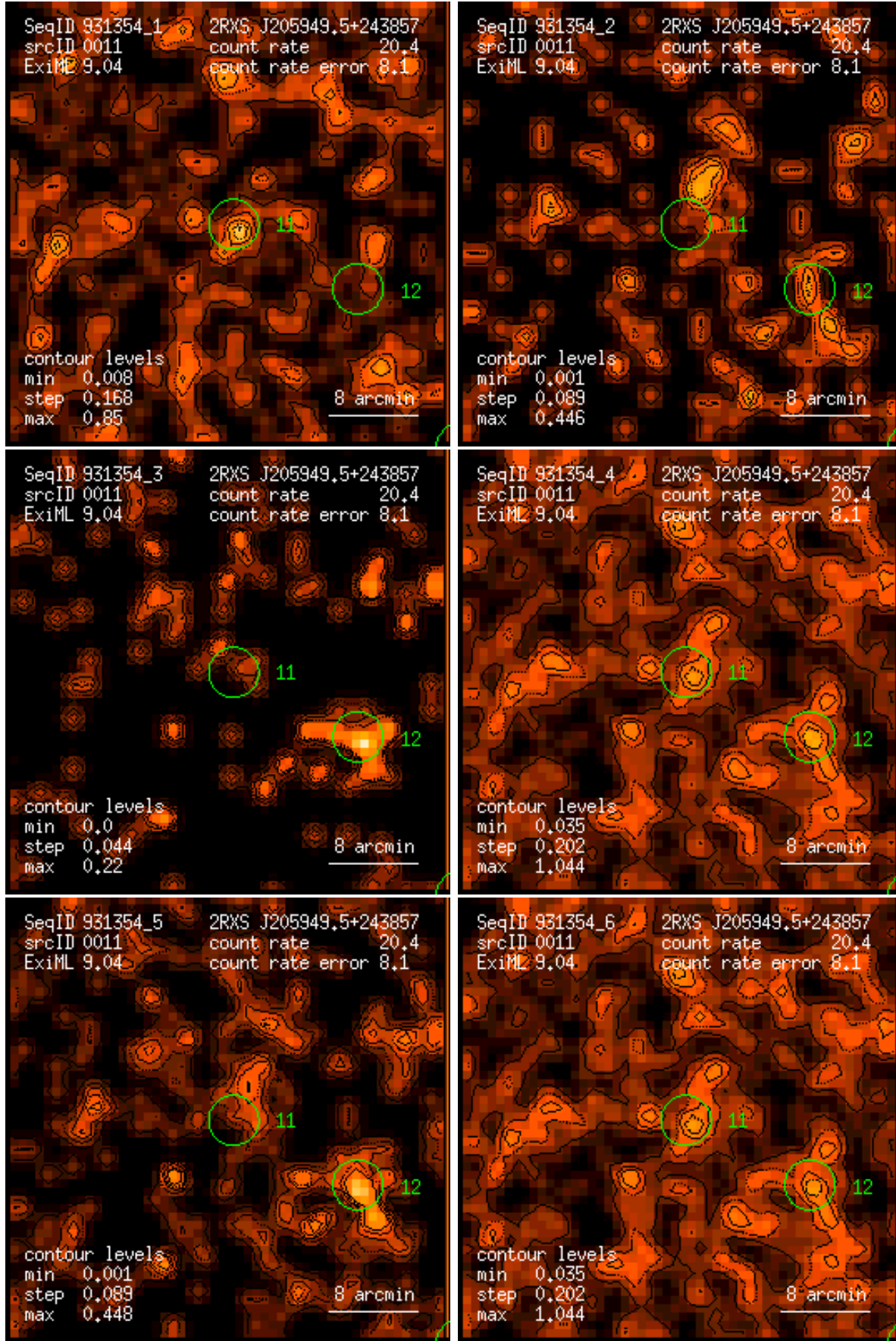
Figure 11: RASS 931354: detection 0011: band rate images, Gaussian filter: (1) PSPC channels 11 – 41, (2) 52 – 90, (3) 91 – 201, (4) 11 – 235, (5) 52 – 201, (6) 11 – 201. Broad band rates in counts/ks. Band rate contour levels in counts/ks/arcmin 2 .
