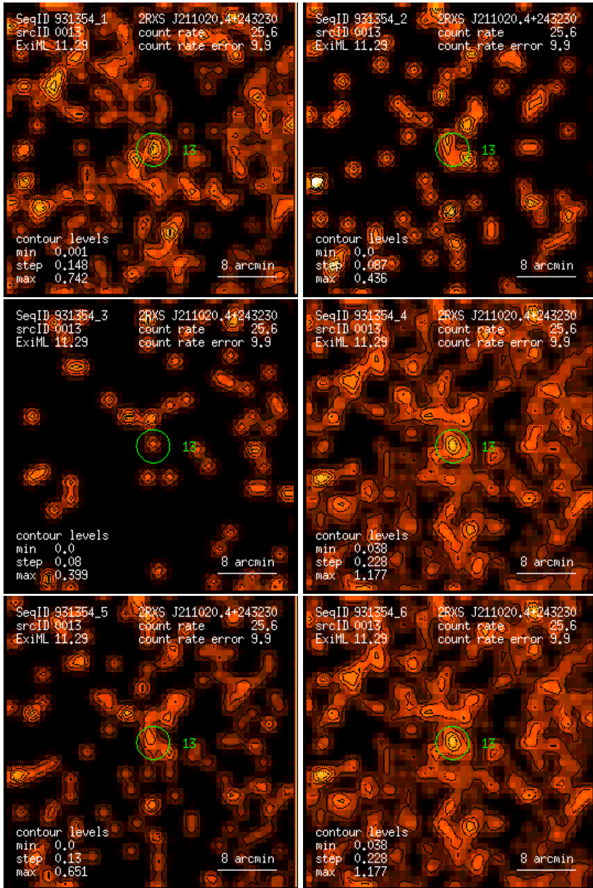
Figure 13: RASS 931354: detection 0013: band rate images, Gaussian filter: (1) PSPC channels 11 – 41, (2) 52 – 90, (3) 91 – 201, (4) 11 – 235, (5) 52 – 201, (6) 11 – 201. Broad band rates in counts/ks. Band rate contour levels in counts/ks/arcmin 2 .
