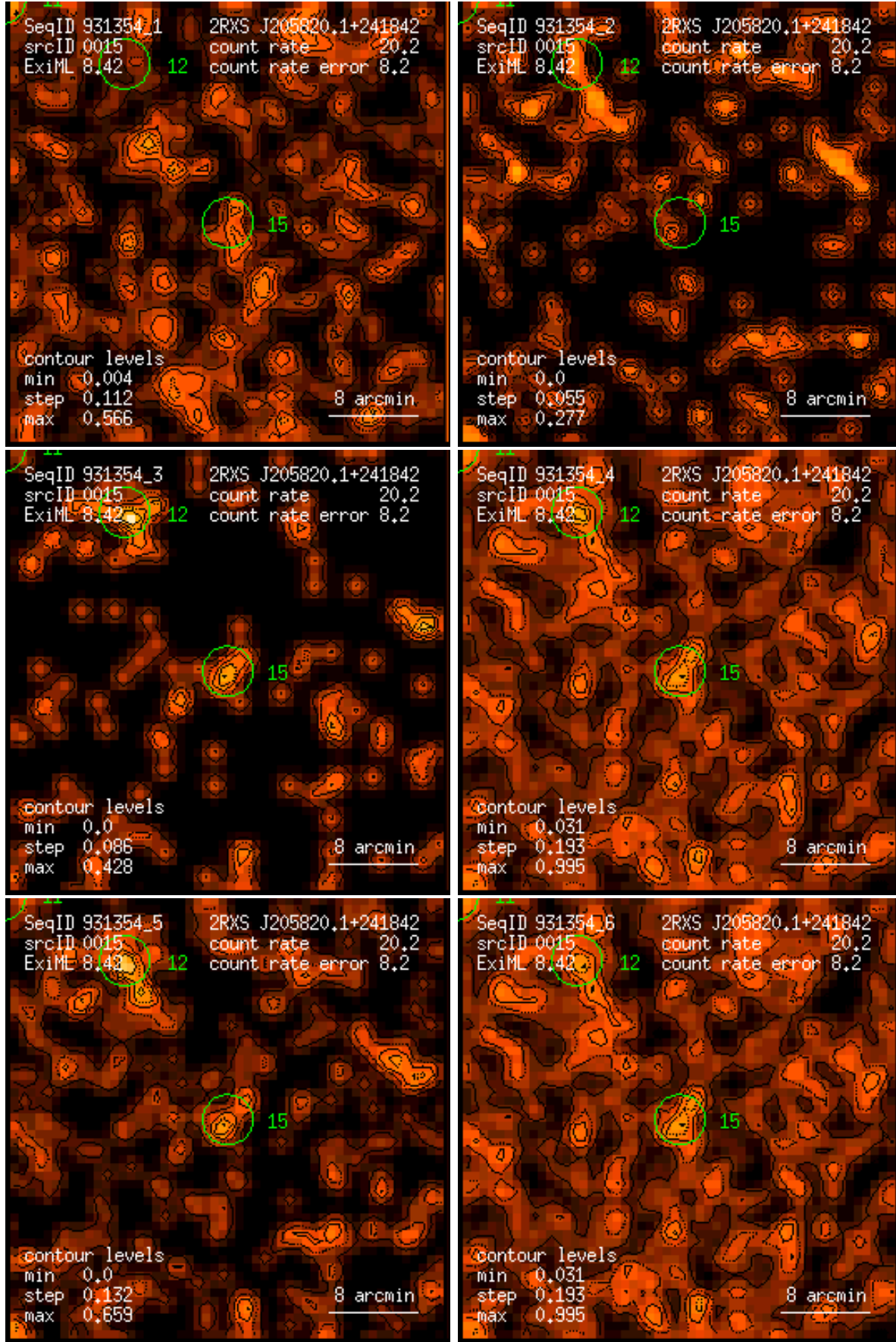
Figure 15: RASS 931354: detection 0015: band rate images, Gaussian filter: (1) PSPC channels 11 – 41, (2) 52 – 90, (3) 91 – 201, (4) 11 – 235, (5) 52 – 201, (6) 11 – 201. Broad band rates in counts/ks. Band rate contour levels in counts/ks/arcmin 2 .
