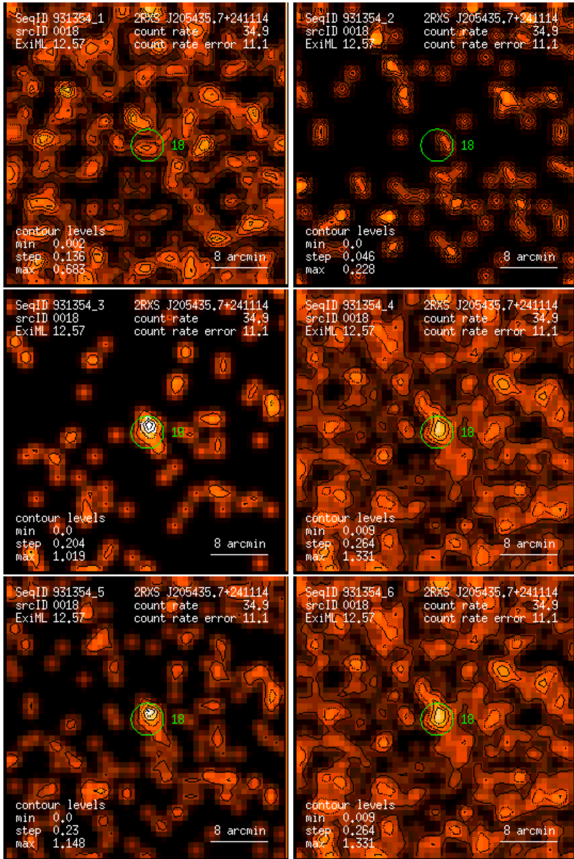
Figure 18: RASS 931354: detection 0018: band rate images, Gaussian filter: (1) PSPC channels 11 – 41, (2) 52 – 90, (3) 91 – 201, (4) 11 – 235, (5) 52 – 201, (6) 11 – 201. Broad band rates in counts/ks. Band rate contour levels in counts/ks/arcmin 2 .
