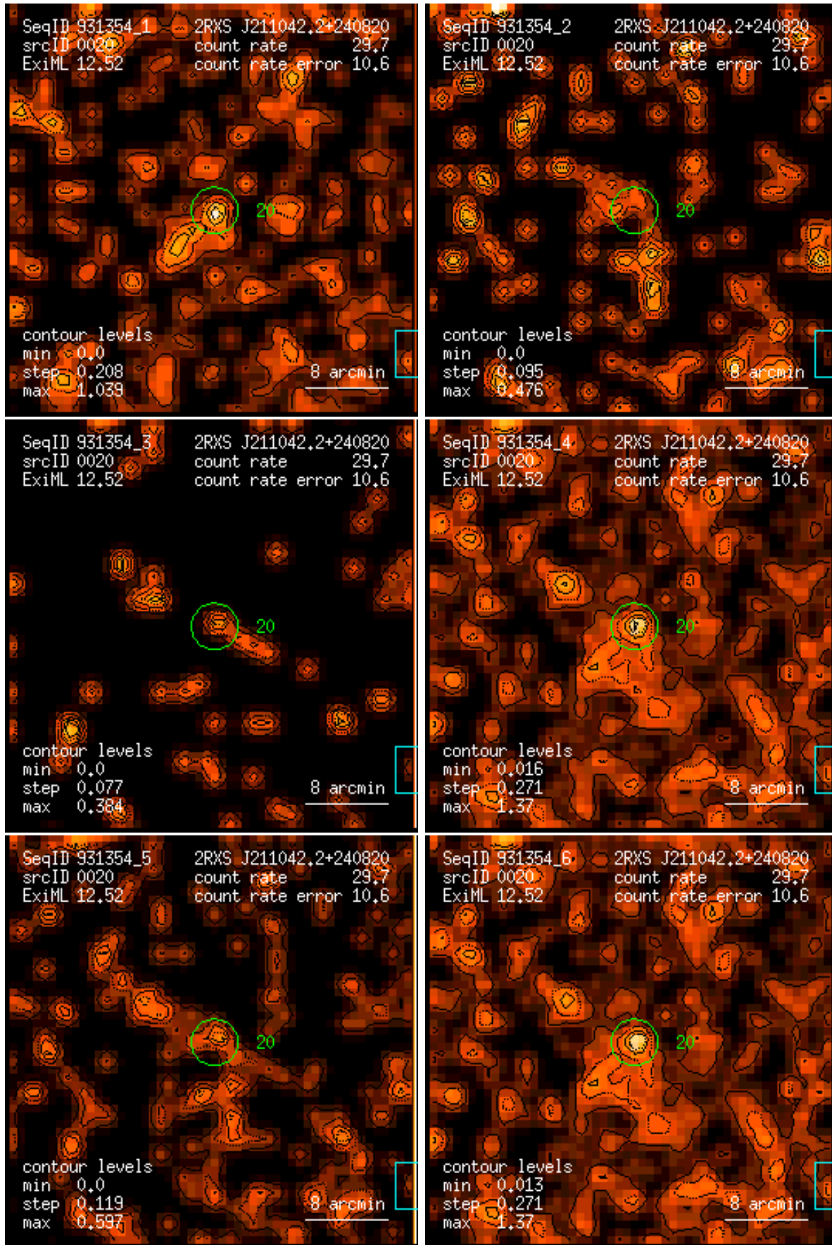
Figure 20: RASS 931354: detection 0020: band rate images, Gaussian filter: (1) PSPC channels 11 – 41, (2) 52 – 90, (3) 91 – 201, (4) 11 – 235, (5) 52 – 201, (6) 11 – 201. Broad band rates in counts/ks. Band rate contour levels in counts/ks/arcmin 2 .
